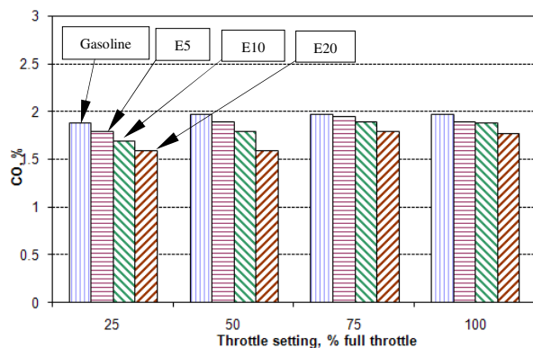
Fig.1.6. Effect of throttle on the CO, at engine speed of 2000 rpm
