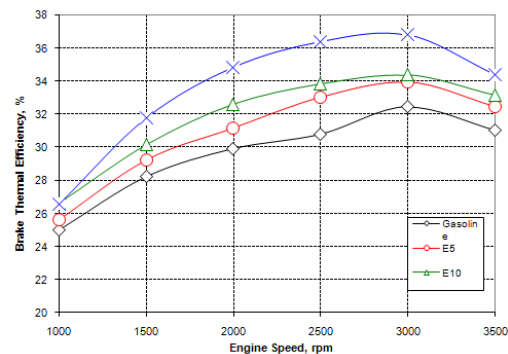
Fig. 1.4. Thermal efficiency versus engine speed, at 25% full throttle
