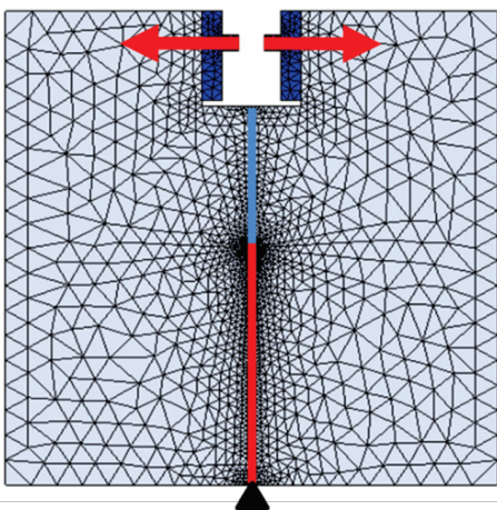
Figure 5: Finite Element mesh and boundary conditions of the problem.
