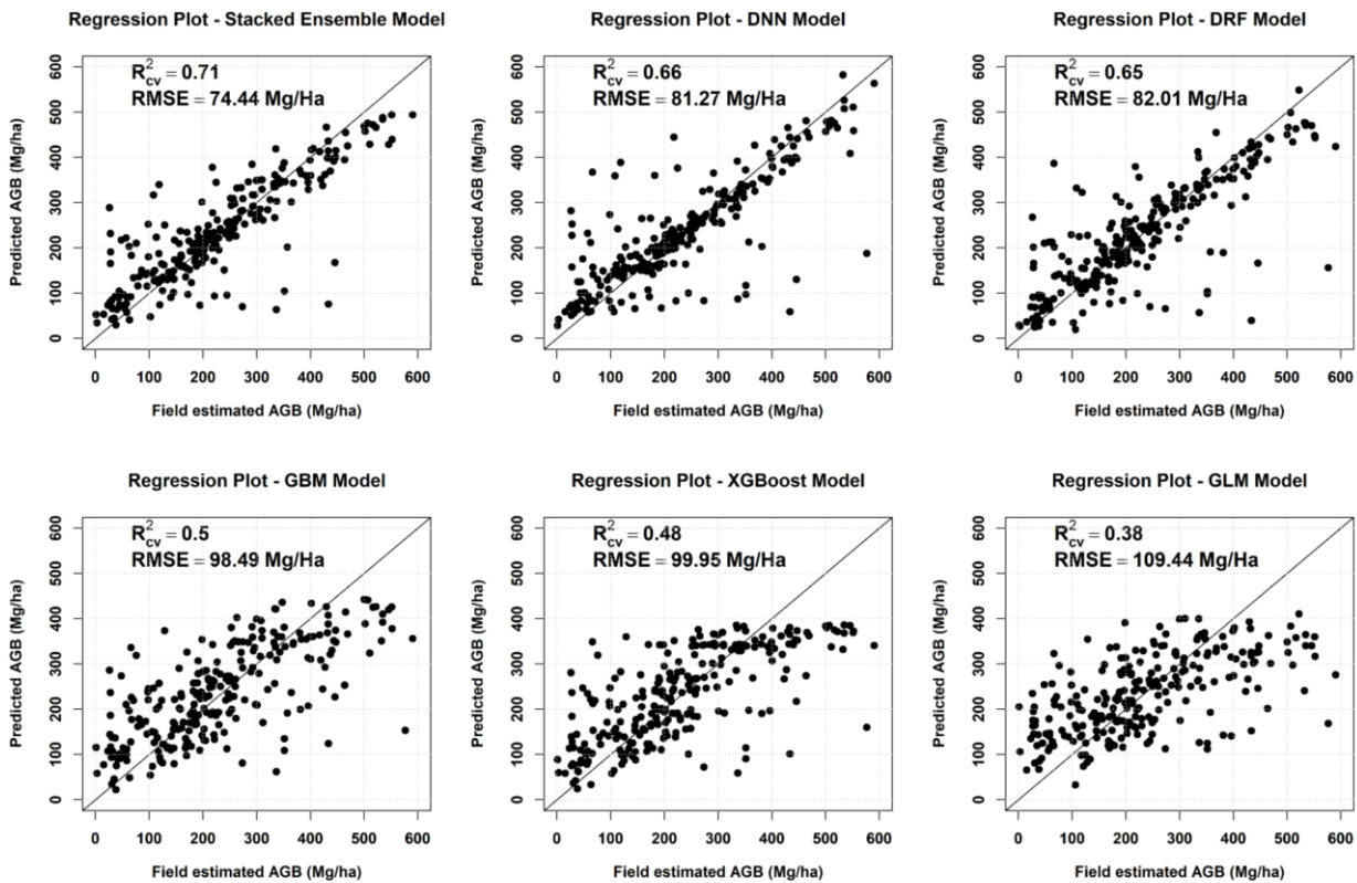
Fig. 4. Regression scatter plots of the considered models
