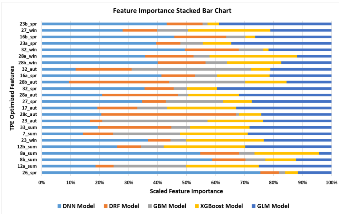
Fig. 3. Feature Importance Stacked Bar Chart
