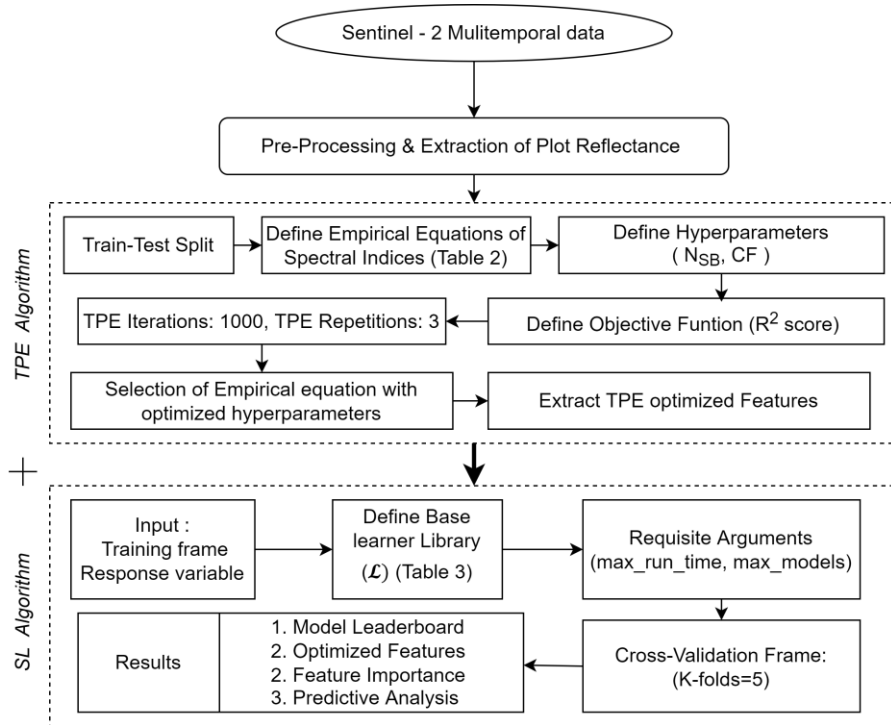
Fig. 2. Proposed Approach for AGB prediction
