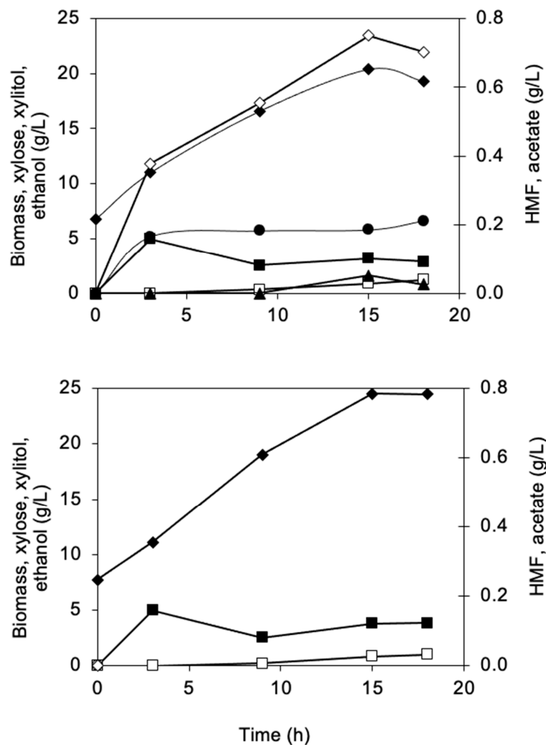
Figure 2. Profile of fed-batch cultivation with S. cerevisiae TMB3500 in spruce hydrolysate (top) and in sugar mixture (bottom). First y -axis: biomass (◆), xylose (■), xylitol (□), ethanol (▲); second y -axis: acetate (◇) and HMF (●). Duplicate experiments showed similar results and the figure shows one of the representative profiles for each cultivation.
