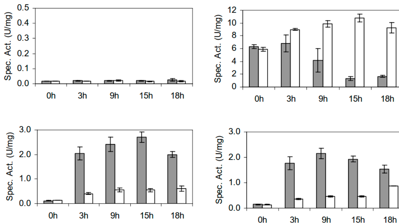
Figure 5. HMF (left column) and furfural (right column) reduction activity measurements in crude cell extracts from yeast cells cultivated in fed-batch mode using either spruce hydrolysate (SH; grey bars) or sugar medium (SM; white bars). Activity was measured using either NADH (top row) or NADPH (bottom row) as cofactor.
