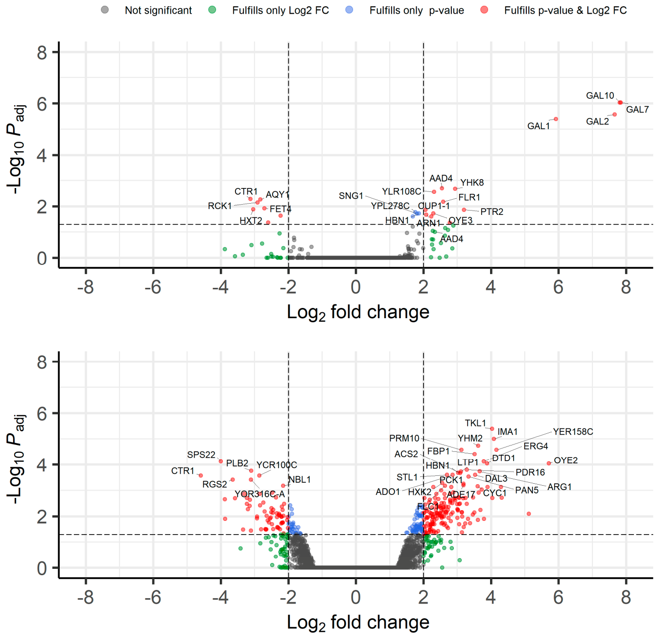
Figure 6. Volcano plots showing the results of the microarray data processed using the “global” settings of Limma’s decideTests. The P_{adj} of the y -axis represents Benjamini–Hochberg adjusted p -values. (A): Comparison of gene expression between spruce hydrolysate 9 h and sugar medium 9 h (SH 9 h vs. SM 9 h). Due to display limitations, only the 20 significant differentially expressed (DE) genes with lowest adjusted p -values from this comparison are labeled. Note that there are two probes on the Affymetrix Yeast Genome 2.0 array annotated as AAD4 and that only one of them (1771716_s_at) was found to be significantly DE by the test. Four genes with an average \log_2 fold change just below the >|2| threshold were found to be statistically significant according to decideTests when the replicates were taken into consideration. (B): Comparison of gene expression between spruce hydrolysate 17 h and sugar medium 17 h (SH 17 h vs. SM 17 h). The 30 significant differentially expressed (DE) genes with lowest adjusted p -values from this comparison are labeled. For this figure, all S. pombe and control probes were omitted, and thus only contain the 5814 S. cerevisiae probes from the Yeast Genome 2.0 array. The full results for all probes can be found in Supplemental Information 2.
