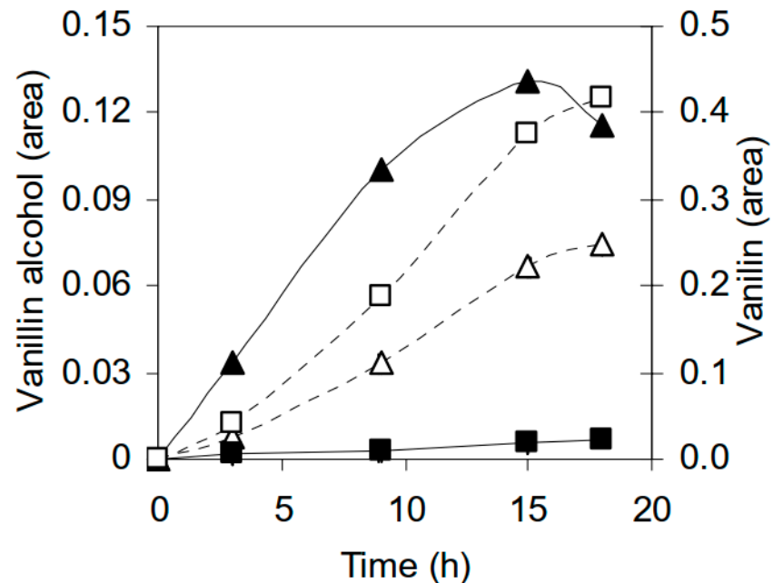
Figure 4. Conversion of vanillin to vanillic/vanillyl alcohol in the fed-batch cultivation of S. cerevisiae TMB3500 in spruce hydrolysate. Filled symbols: measured values; empty symbols: the expected amount considering the amount of hydrolysate added. Compounds: vanillin (■), vanillin alcohol (▲).
