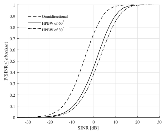
Fig. 4: SINR distributions using different antennas onboard UAVs.
