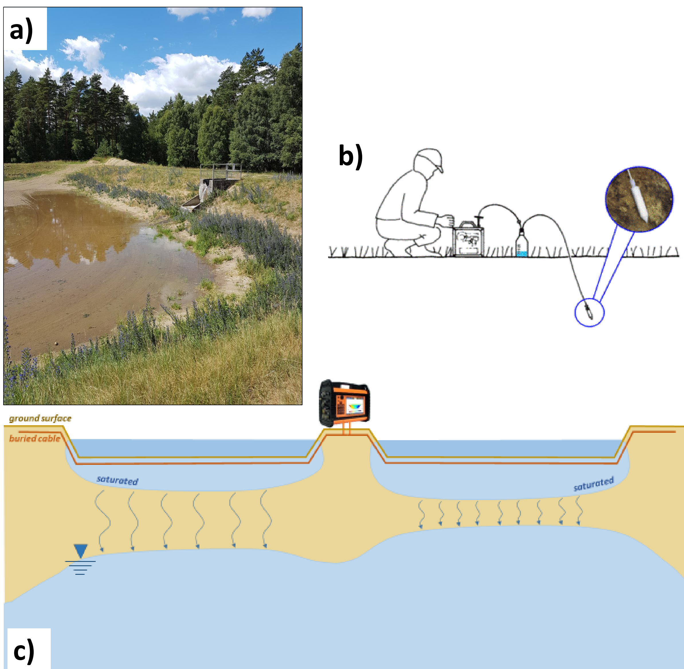
a) Infiltration pond; b) permanent water sampling; c) sketch of DCIP monitoring
