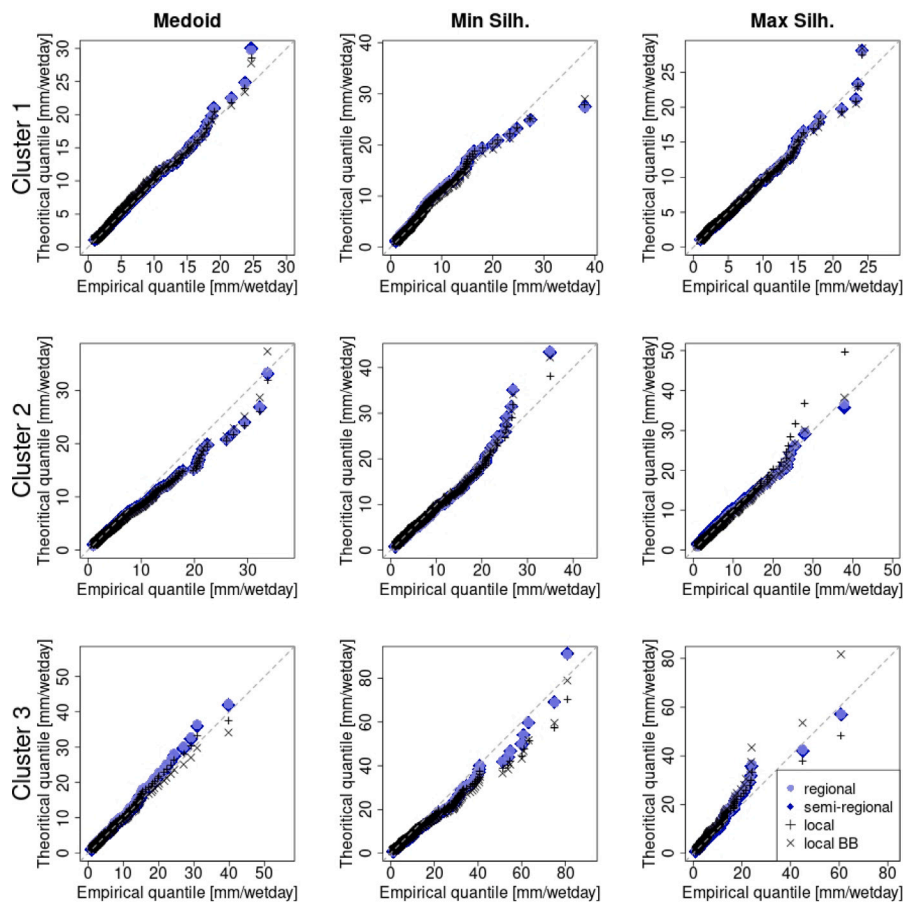
Fig. 2. Example QQ plots of the regional, semiregional, local, and local Bernstein (local BB) fittings, for the medoid point (left) and the grid points with minimum (middle) and maximum (right) silhouettes in the northern (top row), intermediate (middle row), and southern (bottom row) clusters in SON (blue cluster in Fig. 1).
