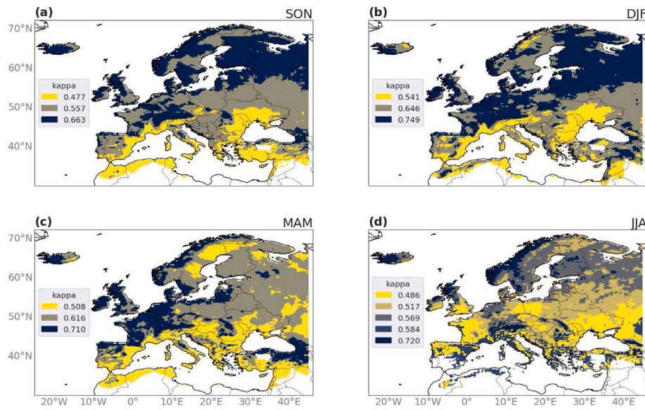
Fig. A.2. Flexibility parameter \kappa for the regional fitting, for the season (a) SON, (b) DJF, (c) MAM and (d) JJA, see last row of Table 1.
