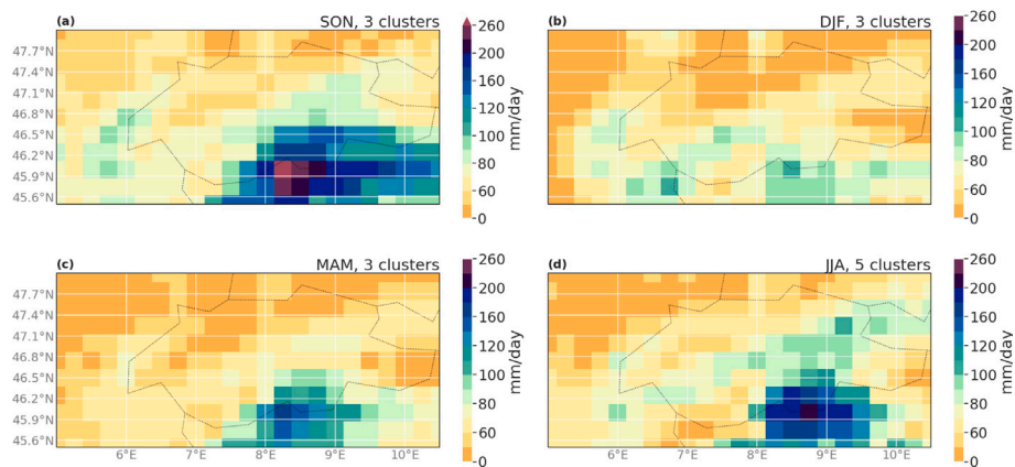
Fig. C.2. 50-year return levels in Switzerland computed with the regional fitting, for a comparison with the one provided by MeteoSwiss (2019) .
