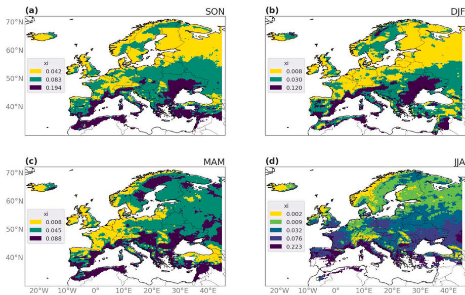
Fig. A.1. Shape parameter \xi for the regional fitting, for the season (a) SON, (b) DJF, (c) MAM and (d) JJA, see last row of Table 1.
