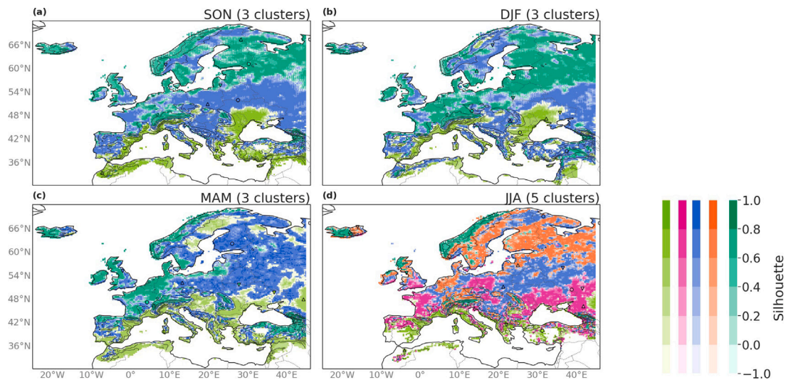
Fig. 1. Partition with the PAM algorithm applied on ERA-5 daily positive precipitation over Europe for all seasons. Each cluster is identified by a colour. The shades of colour indicate the silhouette coefficient at every grid point. Intense hues indicate a strong association with the cluster. The black lines are 500 [m] altitude isolines of the surface topography in ERA-5. Within a cluster, the circle indicates the location of the medoid, and the triangle pointing up (resp. down) indicates the grid point with the highest (resp. lowest) silhouette coefficient.
