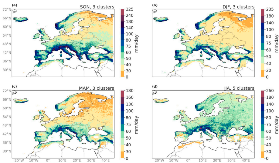
Fig. 5. 100-year return levels computed with the regional fitting, see Table 1.
