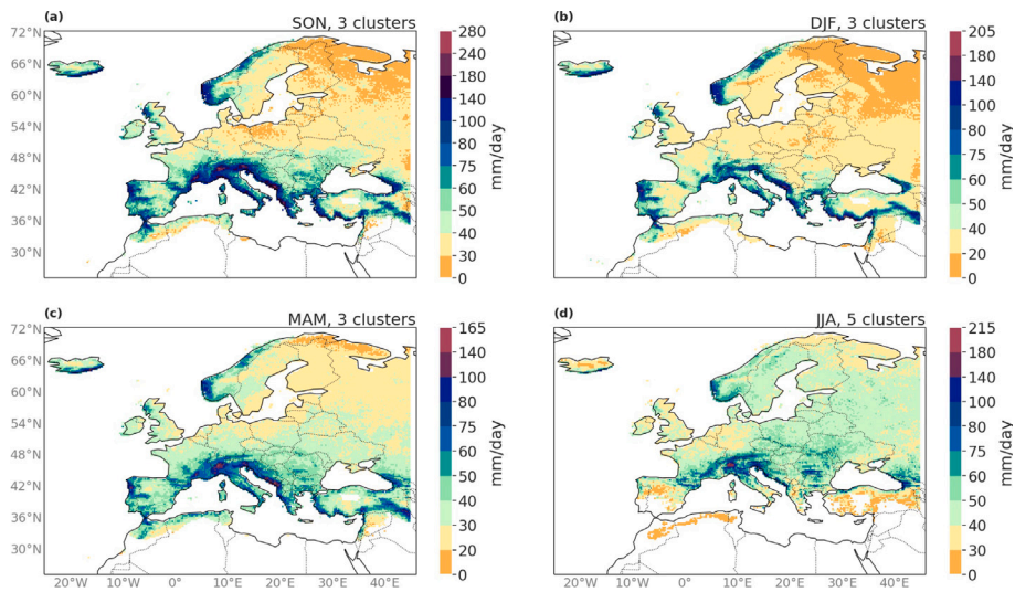
Fig. 4. 50-year return levels computed with the regional fitting, see Table 1.
