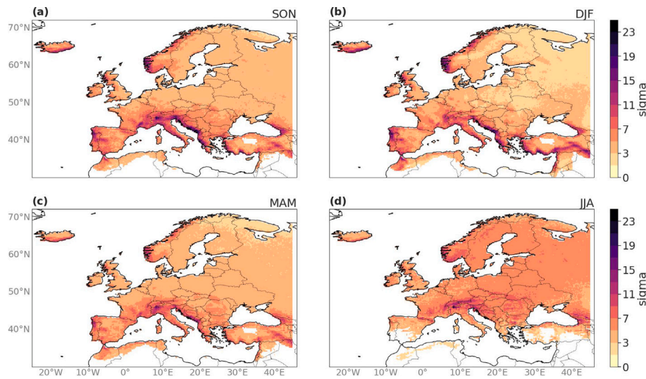
Fig. A.3. Scale parameter \sigma for the regional fitting, for the season (a) SON, (b) DJF, (c) MAM and (d) JJA, see last row of Table 1.
