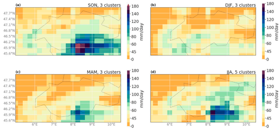
Fig. C.1. 10-year return levels in Switzerland computed with the regional fitting, for a comparison with the one provided by MeteoSwiss (2019) .
