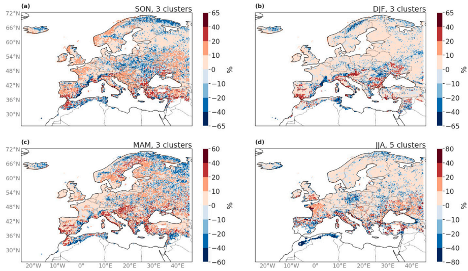
Fig. B.2. Relative difference between the 100-year return levels computed with the regional fitting and the local fitting.
