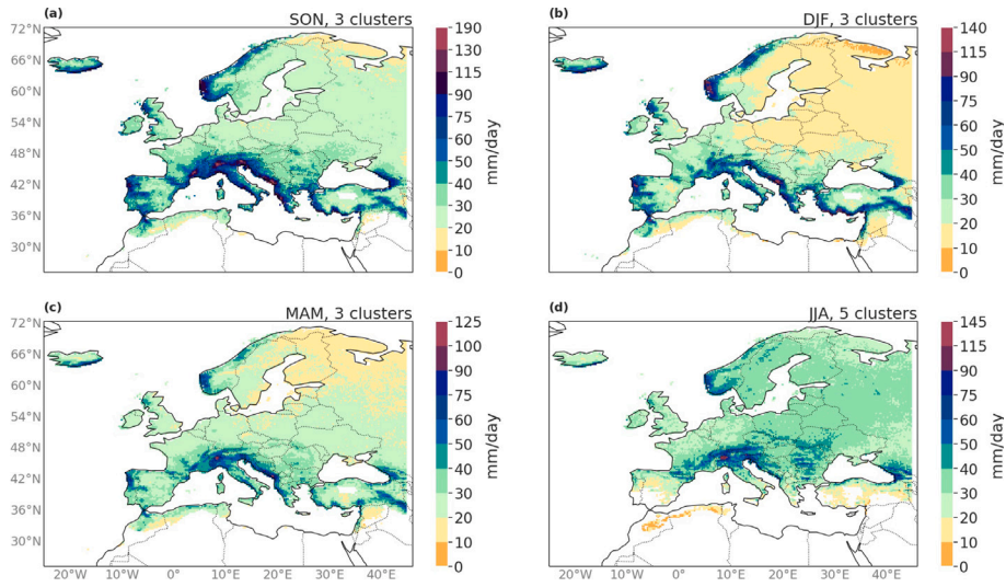
Fig. 3. 10-year return levels computed with the regional fitting, see Table 1.
