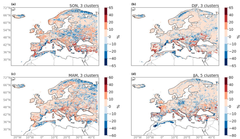
Fig. 6. Relative difference between the 50-year return levels computed with the regional fitting and the local fitting.
