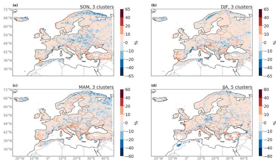
Fig. B.1. Relative difference between the 10-year return levels computed with the regional fitting and the local fitting.
