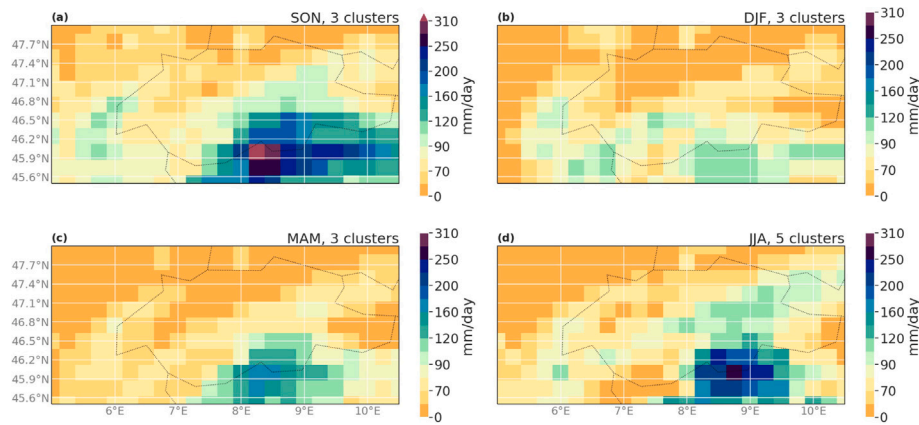
Fig. C.3. 100-year return levels in Switzerland computed with the regional fitting, for a comparison with the one provided by MeteoSwiss (2019).
