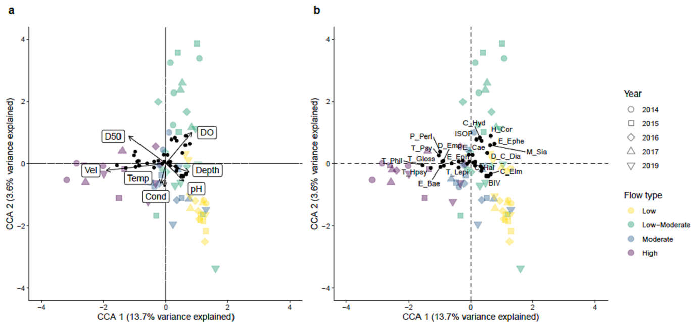
Fig. 2. Canonical Correspondence Analysis (CCA) ordination of A) environmental variables and B) benthic macroinvertebrate abundance data for 72 samples collected along the main stem of the WJSR, with the colour of points indicating the flow category and the shape indicating the year. Arrows denote habitat variables included in the CCA. Axis labels indicate the percent unconstrained variance in the BMI assemblage that is explained by each axis. To facilitate the interpretation of the figure, only a subset of taxa are labelled.
