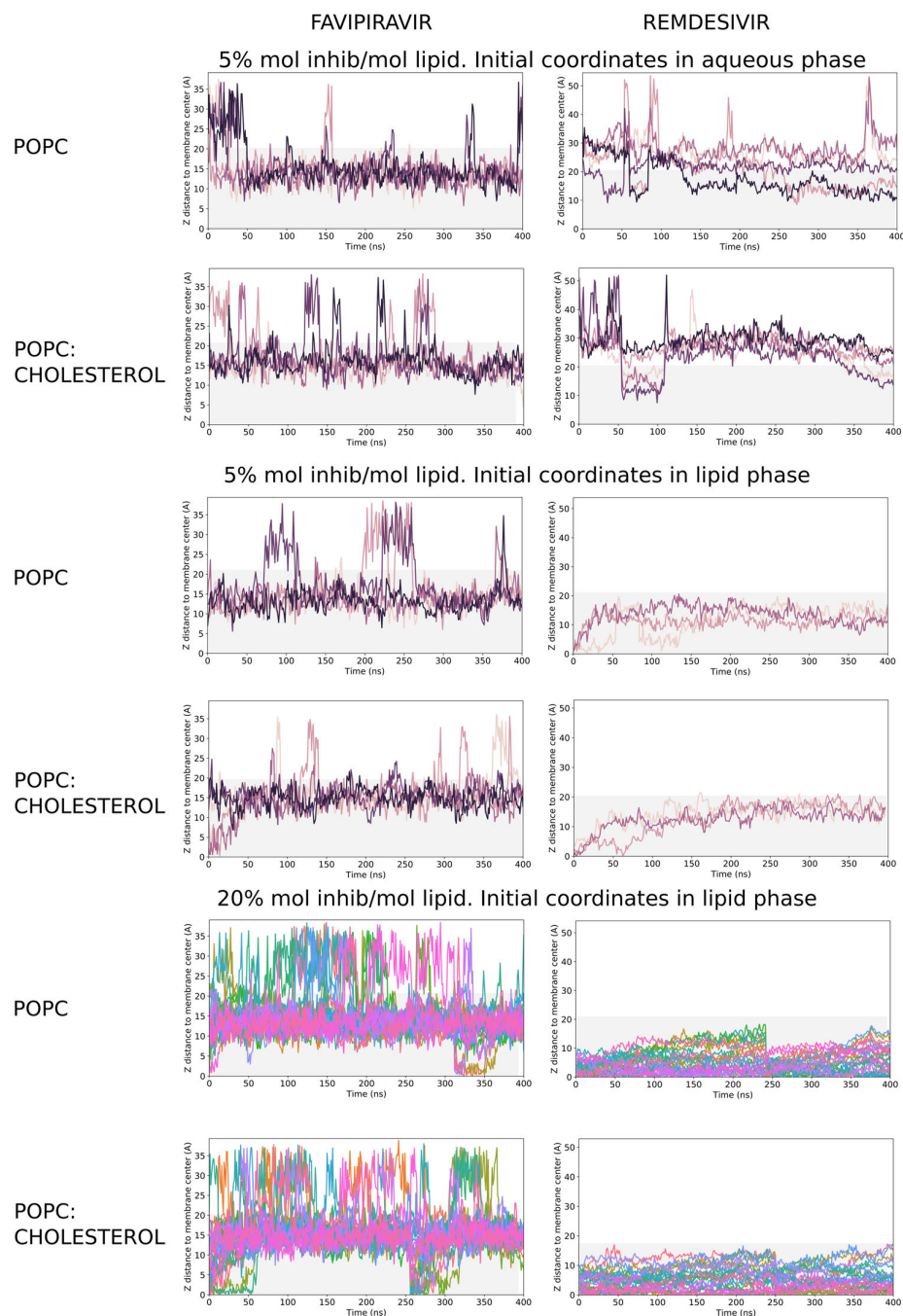
Figure 2. Position of the center of mass as a function of the simulation time of favipiravir (left) and remdesivir (right) molecules in a pure POPC (top) and POPC:Cholesterol (bottom) for both concentration systems with the inhibitor molecules initially in the aqueous phase and lipid phase, as indicated. Regions between phospholipidic polar head groups are shaded in gray. Each different colored line in each plot represents the course of one inhibitory molecule during the simulation time scale of one replica (400 ns simulation production). The other two replicas are presented in the Supplementary Materials, Figures S3 and S4.
