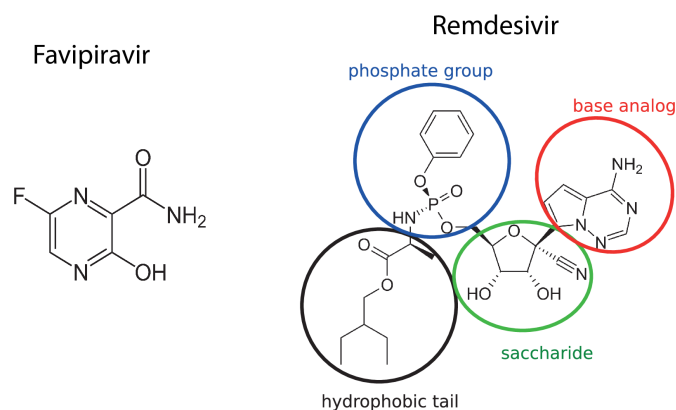
Figure 1. Chemical structure of favipiravir and remdesivir.
