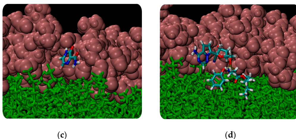
Figure 4. (a) Orientation of favipiravir with respect to the bilayer normal in the POPC (c) and POPC:Cholesterol (d) membranes. Zero degrees means that the O group points towards hydrophilic heads; (b) orientation of the different regions of remdesivir, as defined in Figure 1. Three different vectors as described in the figure are used for proper description.
