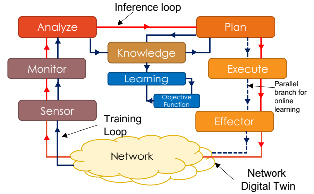
Fig. 3: Extended N-MAPE-K abstractions for NI algorithms example, a NIS could be composed of a Learning-type NIF sending decisions to an engineered model NIF, which acts on the underlying infrastructure.
