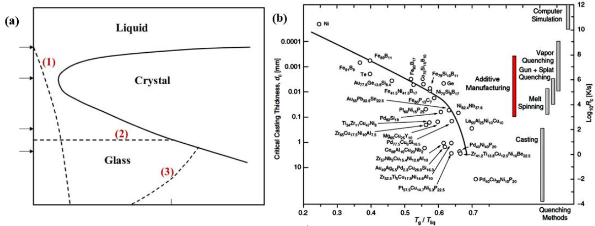
Figure 7: Schematic illustration (a) TTT diagram showing growth of crystal in an under melt phase (1), glass formation due to rapid cooling (2), crystallisation at time t_x due to glass isothermal heat treatment and crystallisation T_x due slowly glass heating (b) Relationship between reduced transition temperature ( T_g/T_m ), critical cooling rate ( R_c ) and critical casting thickness for the MGs and BMGs [180-182]
