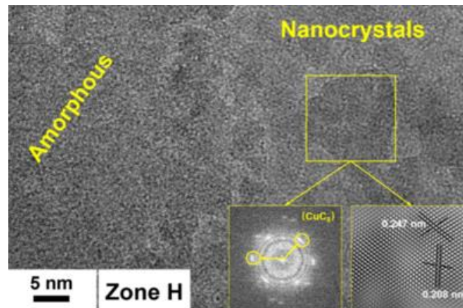
Figure 22: HRTEM micrographs showing microstructure of the partially crystallized Fe-based BMG processed PBF-LB/M indicating the amorphous and nanocrystals phases [289]
