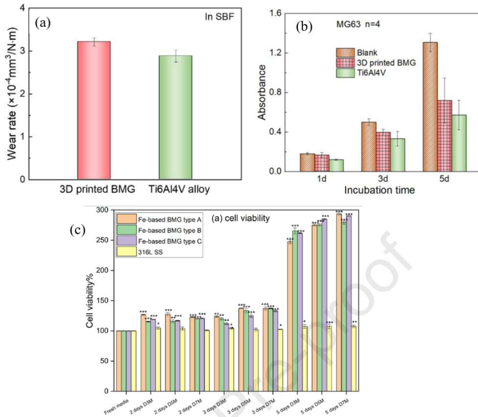
Figure 17: (a) Wear rate of 3D printed BMG and Ti6Al4V alloy observed at 37^\circ in a simulated body fluid (b) Cytotoxicity test of 3D printed BMG and Ti6Al4V alloy using MG63 cell showing the level of absorbance for 1 – 5 days (c) cells viability of three different types of 3D printed Fe-based BMGs compared to 316L stainless steel cultured in SAOS2 cells media for 2, 3 and 5 days [133, 321].
