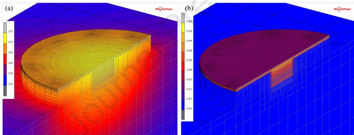
Figure 8: Finite element BMG simulation through PBF-LB/M AM showing (a) 3D contour plot temperature field at one second after deposition of the 50 th layer (b) phase model prediction of the crystalline fraction [231]
