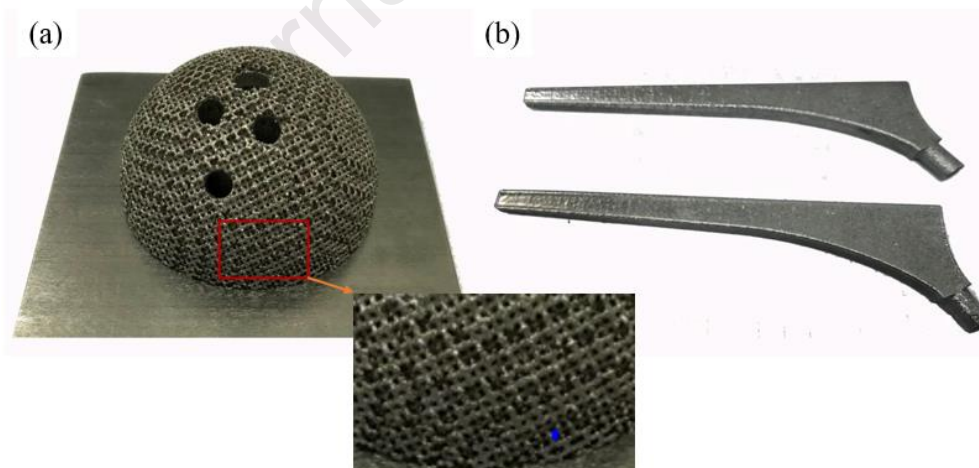
Figure 14: Zr-based BMG 3D printed implants fabricated by PBF-LB/M process (a) acetabular cup with corresponding pores topology (b) femoral components [289]
