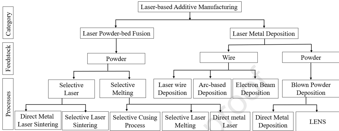
Figure 3: Various classifications and phases of laser-based additive manufacturing
