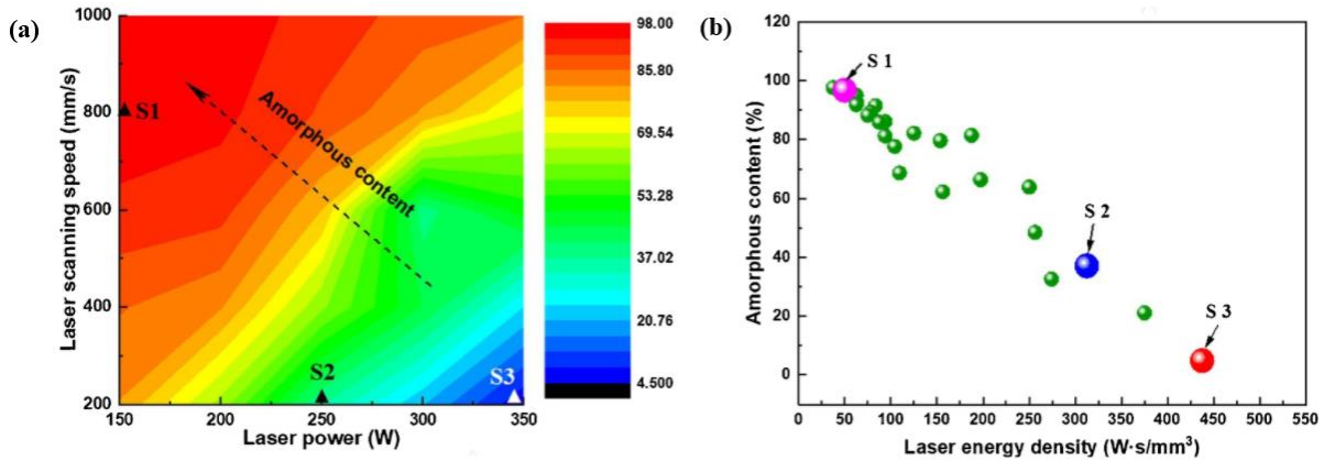
Figure 12: Influence of process parameters on amorphous contents of the Fe-based BMG processed through PBF-LB/M process (a) A map relating scanning speed, laser power and amorphous contents (b) LE verses amorphous contents
