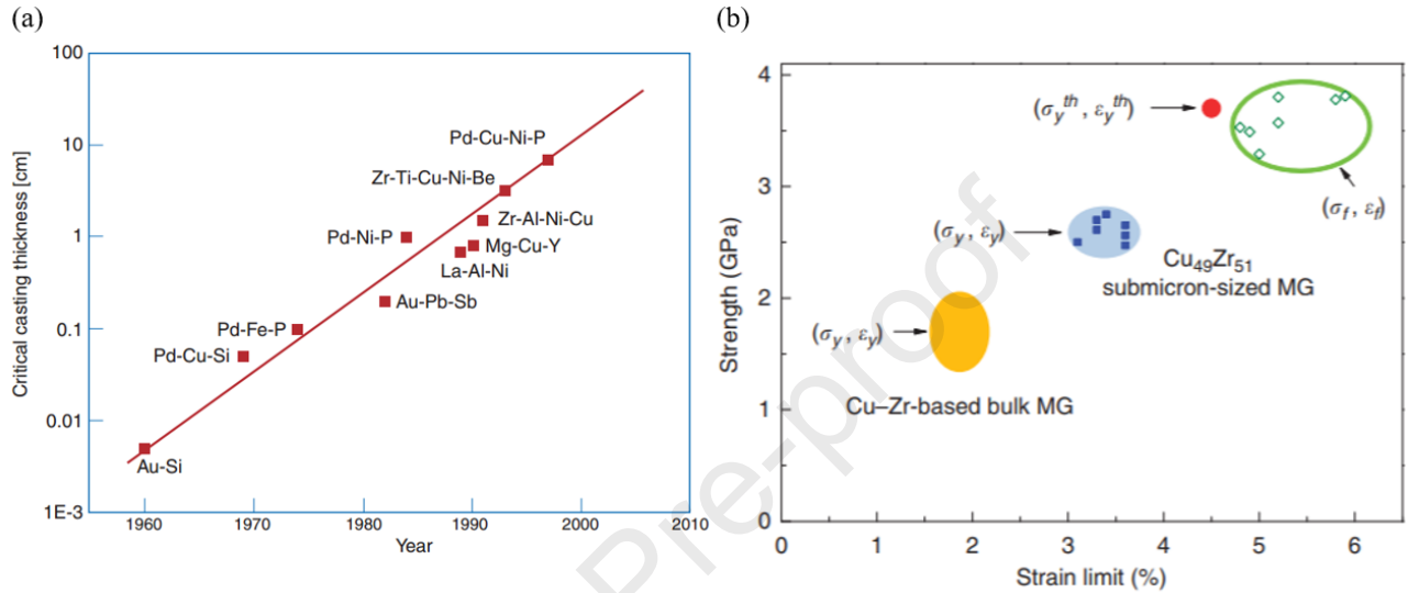
Figure 1: (a) Various varieties of BMGs indicating year of its discovery versus the critical casting size for the amorphous formation (b) Comparison of the small binary and bulk Cu-Zr BMG elastic strain and the corresponding stresses. The strain rate and stresses of the bulk Cu-Zr MGs is indicated by the yellow solid ellipse while the yield strain and strength are of the small MGs is donated by the green square solid. The measured fracture strength and the fracture strain are presented by the blue open diamond [22, 39]
