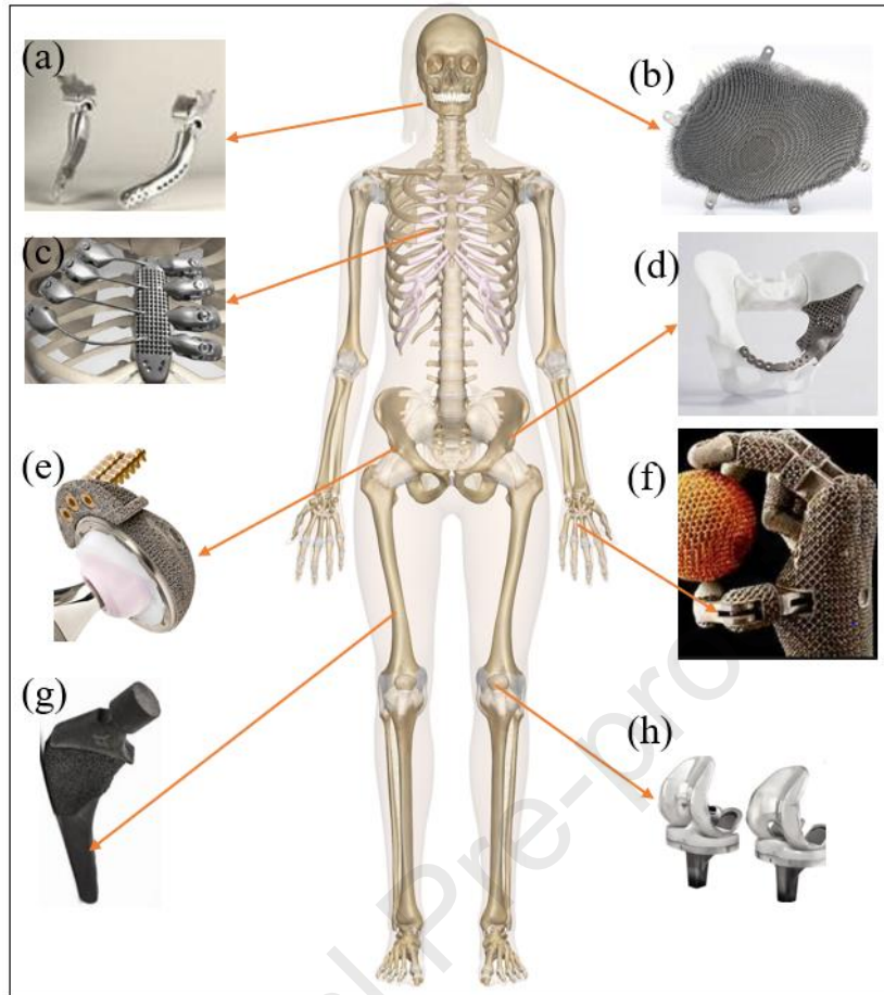
Figure 4: Various implants processed through PBF-LB/M AM process (a) jaw implant [116] (b) cranial implant [117] (c) ribs and sternum [118] (d) pelvic implant [119] (e) hip cup implant [120] (f) hand and toes implants [121] (g) hip implant [122] (h) knee implant [123]
