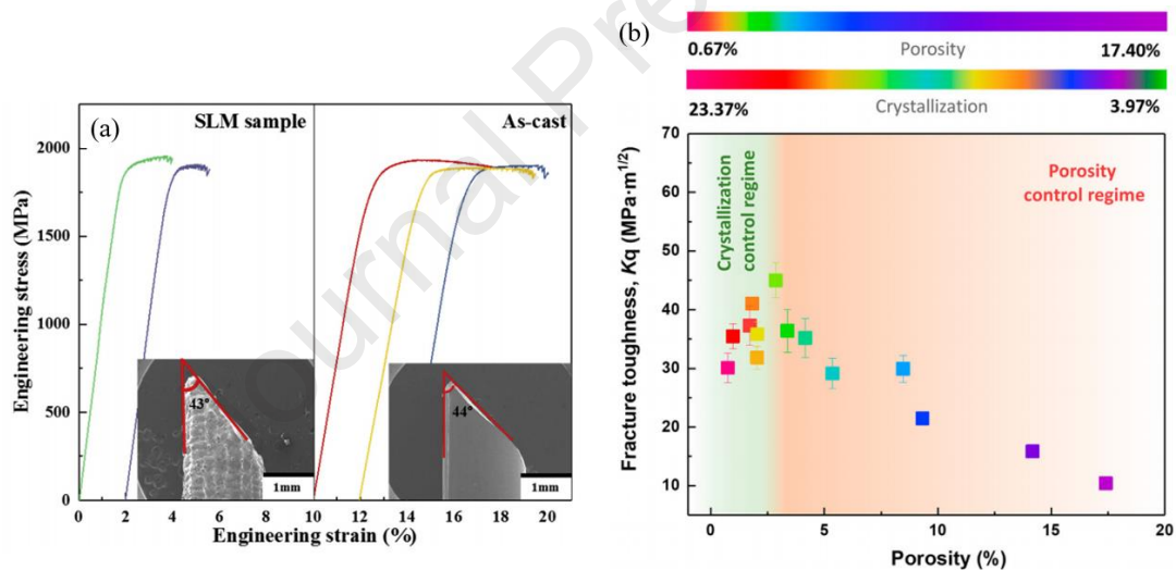
Figure 16: PBF-LB/M processed BMGs (a) compressive stress-strain curve and the plane of fracture compared with the as-cast BMGs (b) fracture toughness at different crystallization fractions and porosities [291, 320]
