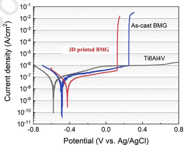
Figure 20: Electrochemical polarization curves of PBF-LB/M processed BMG specimens at 37°C in simulated body fluids compared to as-cast BMG and Ti6Al4V alloy [133].
