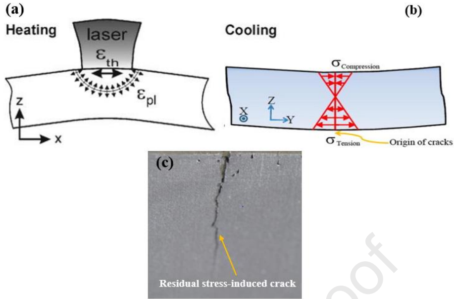
Figure 9: Schematic illustration of the thermal stress behaviour (a) mechanism of temperature gradients (b) position of cracks in PBF-LB/M processed part (c) microstructure of the 3D printed part indicating residual stress-induced crack [238, 239]
