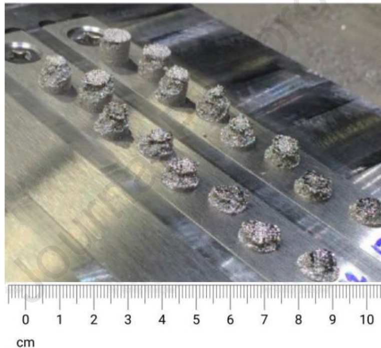
Figure 11: Photograph of the FeCrMoCB BMG specimens processed during initial parameters selection
