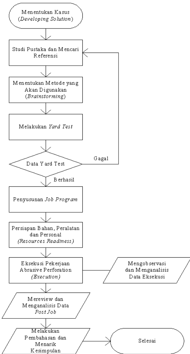
GAMBAR 2. Diagram alir kegiatan abrasive perforation
