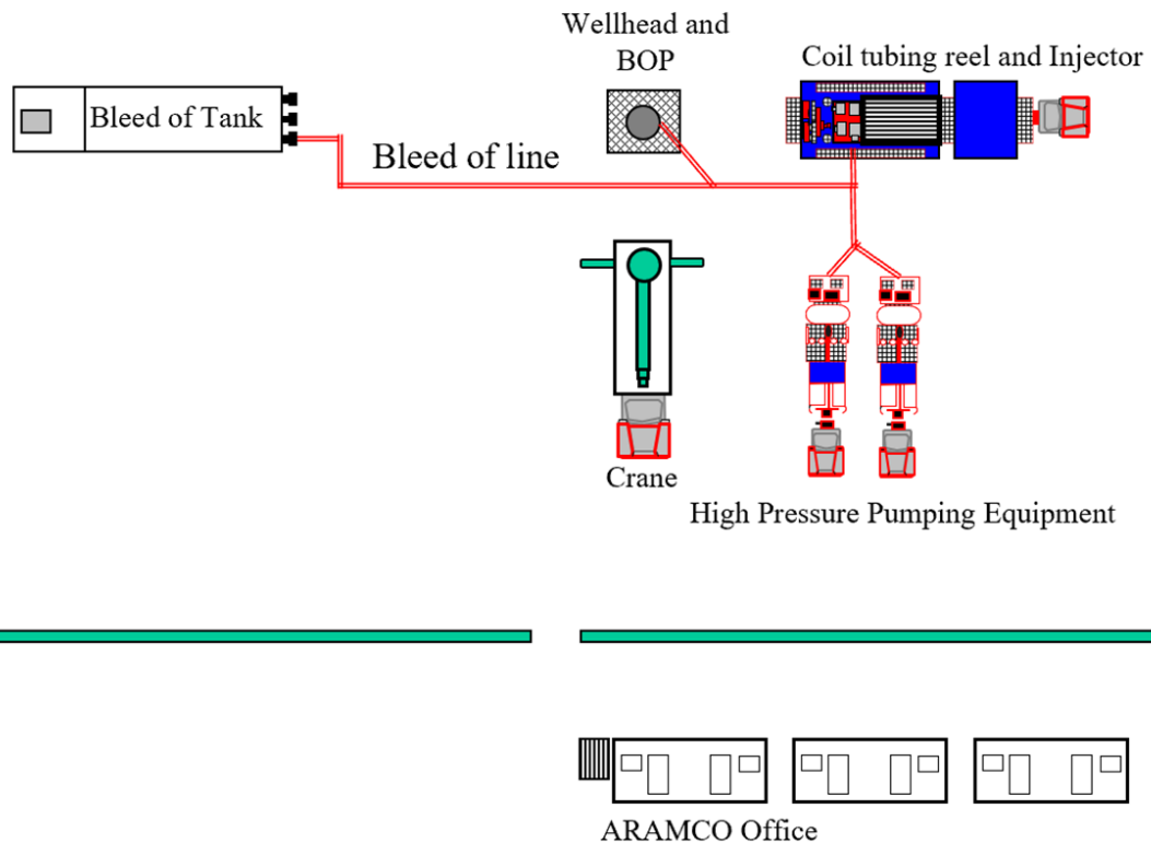
GAMBAR 1. Coil tubing unit set up
