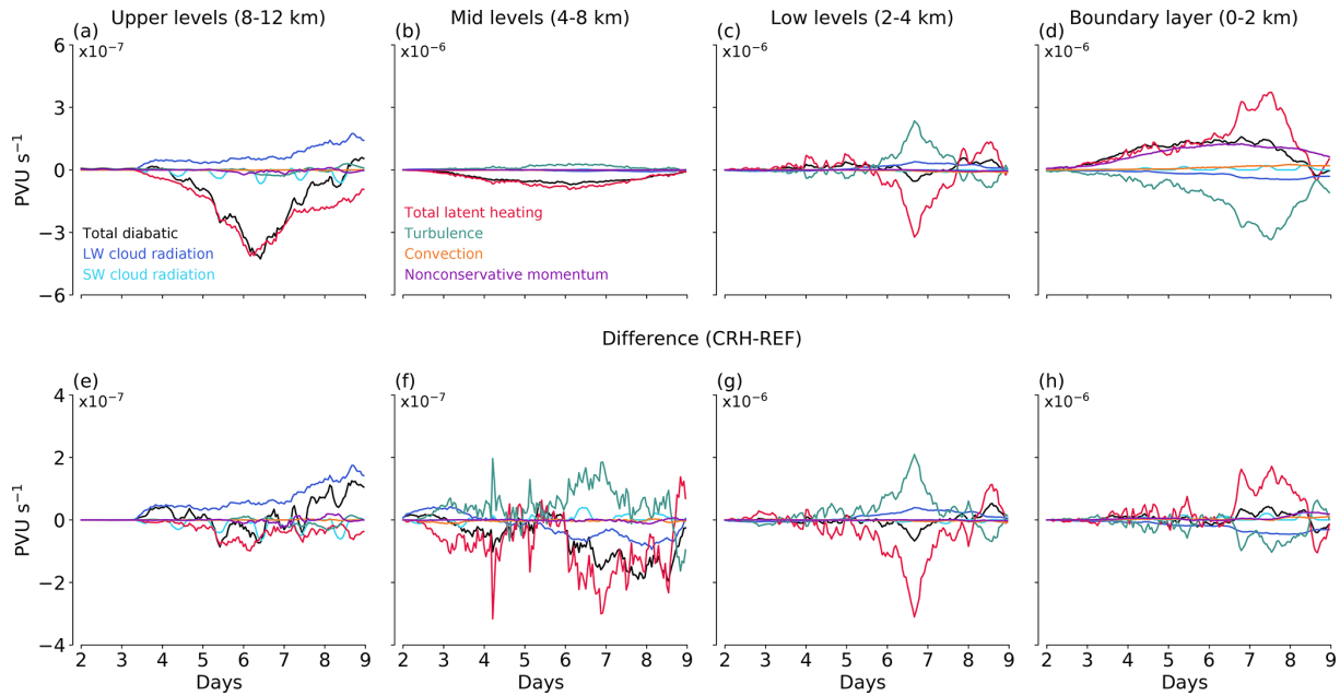
Figure 8. Evolution of spatially averaged and mass-weighted vertical average of diabatic PV tendencies between (a) 8–12 km, (b) 4–8 km, (c) 2–4 km and (d) 0–2 km in the CRH simulation. Panels (e)–(h) show the differences between the CRH and REF simulations (CRH–REF). Note the different y axes in the panels. Total diabatic PV tendency (black line) is the sum of the individual diabatic PV tendencies shown as colored lines.
