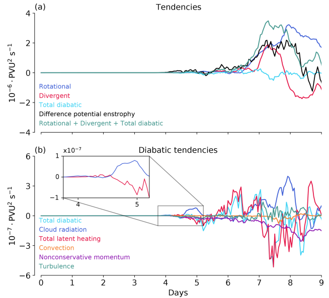
Figure 10. Evolution of the (a) spatially averaged difference potential enstrophy tendency and contributions from individual processes diagnosed from the r.h.s. of Eq. (8). The analysis is performed around the tropopause on the 326 K isentropes. Panel (b) further decomposes the total diabatic (cyan line) contribution into the contributions from individual diabatic processes. Note the different scales in panels.
