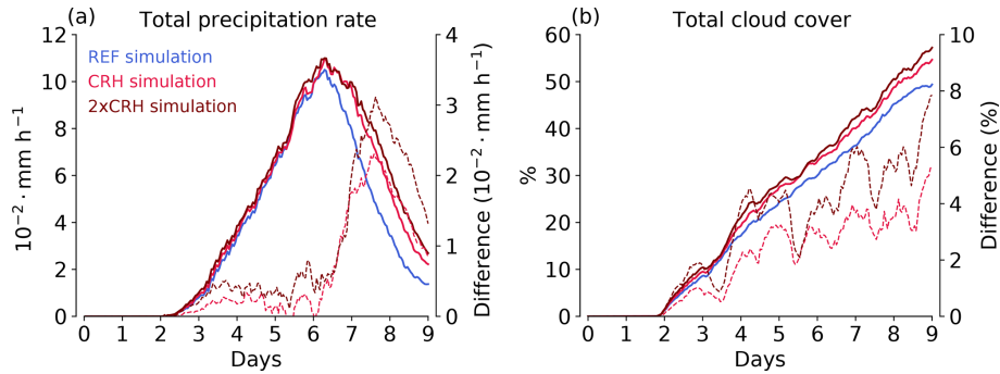
Figure 4. Evolution of spatially averaged (a) total precipitation rate and (b) total cloud cover for different treatments of cloud-radiative heating. The dashed lines denote the differences of the CRH and 2xCRH simulations with respect to the REF simulation. For the differences, the right y-axis is used.
