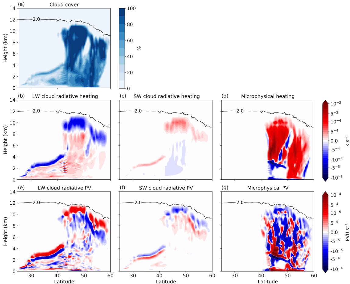
Figure 6. Cross-section through the warm conveyor belt shown in Fig. 1 at day 5.5 for the simulation with CRH. (a) Cloud cover, (b) longwave CRH, (c) shortwave CRH and (d) heating from cloud microphysical processes. Panels (e), (f) and (g) show the associated diabatic PV tendencies. Black contours show the tropopause by the 2 PVU contour.
