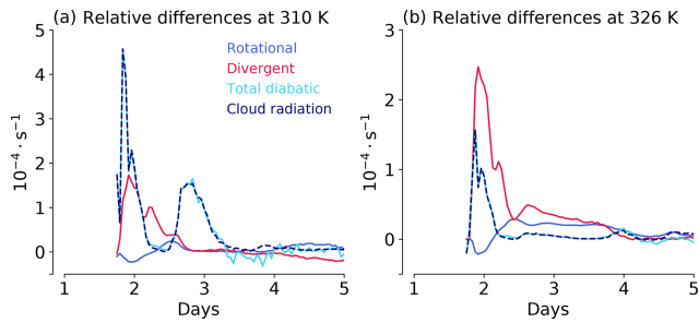
Figure 11. Contribution to the relative growth of difference potential enstrophy from the rotational and divergent flow as well as from total diabatic processes and cloud-radiative heating. Panel (a) is for the 310 K isentrope, which is in the lower troposphere. Panel (b) is for the 326 K isentrope, which is near the tropopause.
