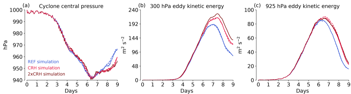
Figure 3. Evolution of (a) cyclone central pressure and eddy kinetic energy at (b) 300 hPa and (c) 925 hPa for simulations with no radiation (REF), cloud-radiative heating (CRH) and cloud-radiative heating increased by a factor of 2 (2xCRH). The dashed lines show additional simulations that use the two-moment instead of the one-moment microphysical scheme.
