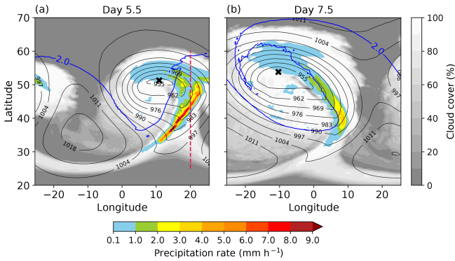
Figure 1. Surface pressure (black contours, hPa), total precipitation rate (colors) and cloud cover (gray shadings) for the cyclone simulation without radiation at (a) day 5.5 and (b) day 7.5. The blue contours indicate the dynamical tropopause as given by the 2 PVU contour on the 326 K isentrope. The dashed red line shows the position of the cross-section shown in Fig. 6. The cross shows the position of the cyclone center given by the minimum surface pressure.
