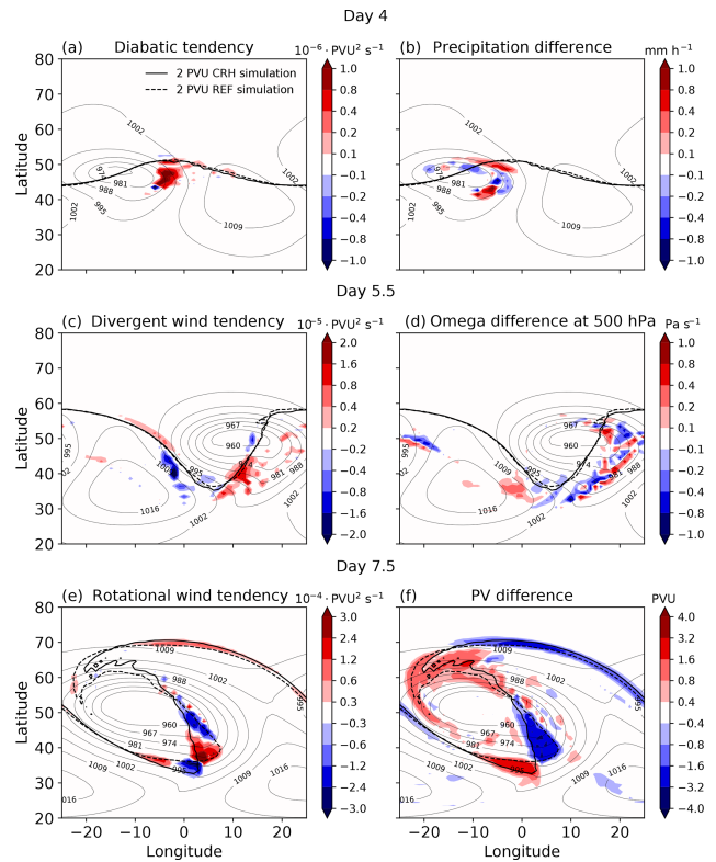
Figure 12. Illustration of the dominant contributions to the evolution of difference potential enstrophy during different stages of the cyclone growth (a, c, e). Panels (b), (d), (f) illustrate the underlying processes by means of fields that are closely related to the different contributions. Thick black contours show the dynamical tropopause for the REF (dashed) and CRH (solid) simulations. Thin contours show the surface pressure (hPa) averaged between the two simulations. The differences are calculated as CRH–REF.
