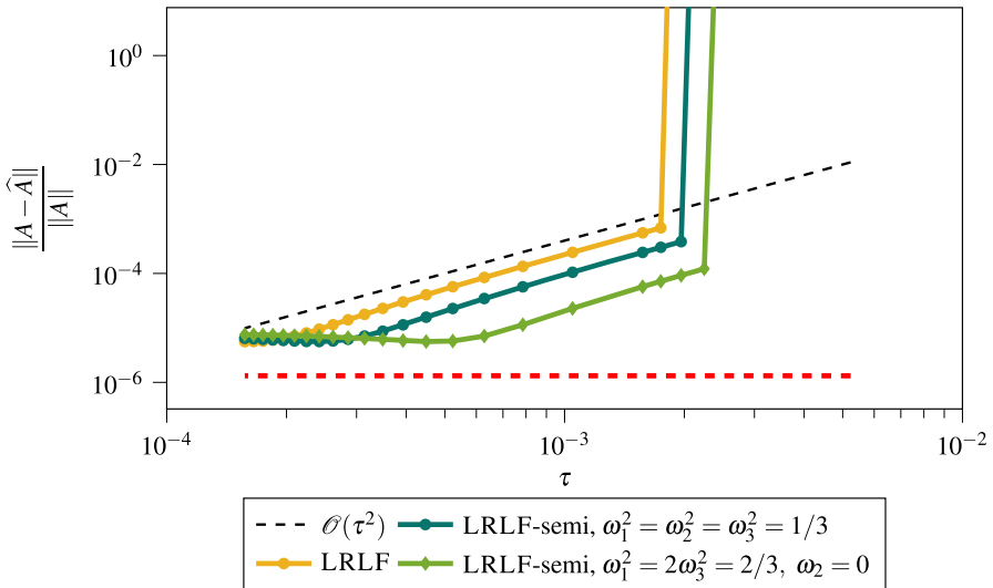
Fig. 2 Example from Sect. 6.2: Relative error in the Frobenius norm between the reference solution of (35) with f given in (39) and the low-rank approximations computed by LRLF and LRLF-semi at time t = 0.5\pi . The red dashed line shows the relative best-approximation error, cf. (40)
