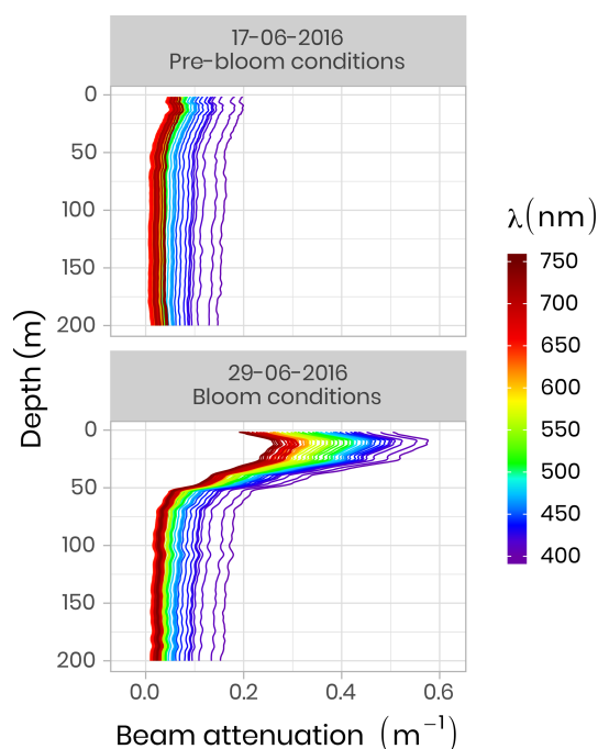
Figure 7. Beam attenuation coefficients ( c , m^{-1} ) measured in 2016 using a WetLabs AC-S before and during the phytoplankton bloom. Note that the colors of the lines correspond to wavelength frequencies.
