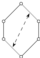
Figure 3. The grey edges represent perspective covers.
