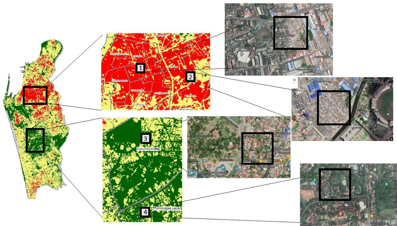
Figure 5. Selected locations for estimation of heat risk reduction. Note: Please refer to Figure 8 for heat risk categories (green = 'low,' yellow = 'moderate' and red = 'high'). The image on left is identical to the heat risk map of Colombo in Figure 8. The purpose is to contextualise the selected locations.
