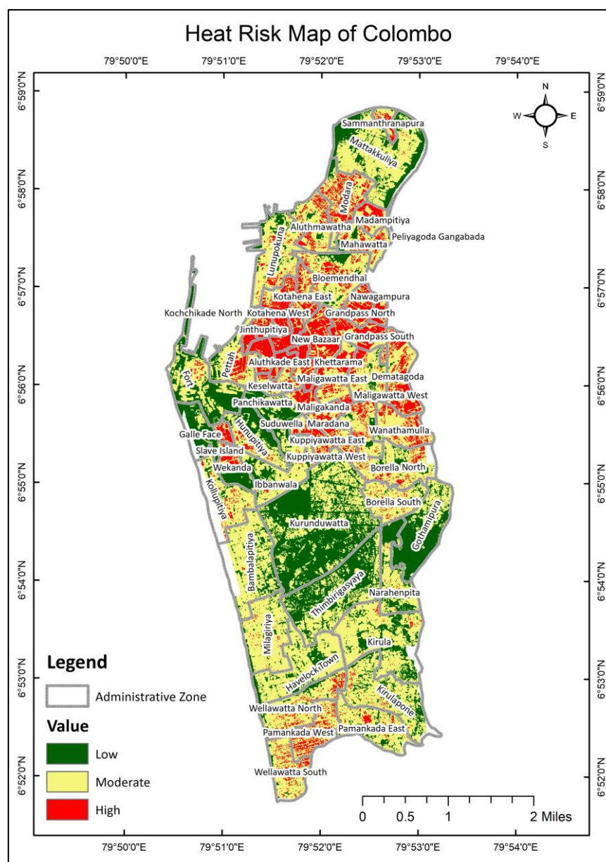
Figure 8. Heat risk map for Colombo, Sri Lanka.
