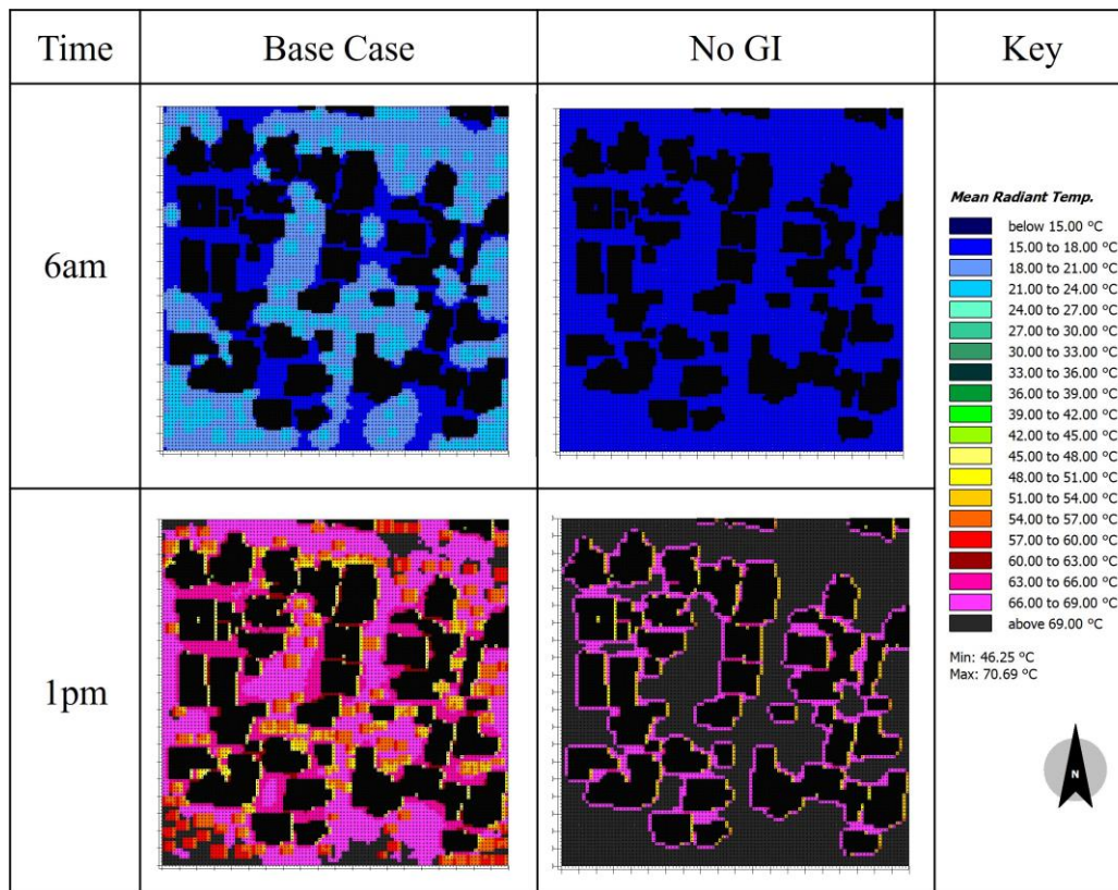
Figure 12. Spatial MRT variations at location 3 for 6 a.m. and 1 p.m.
