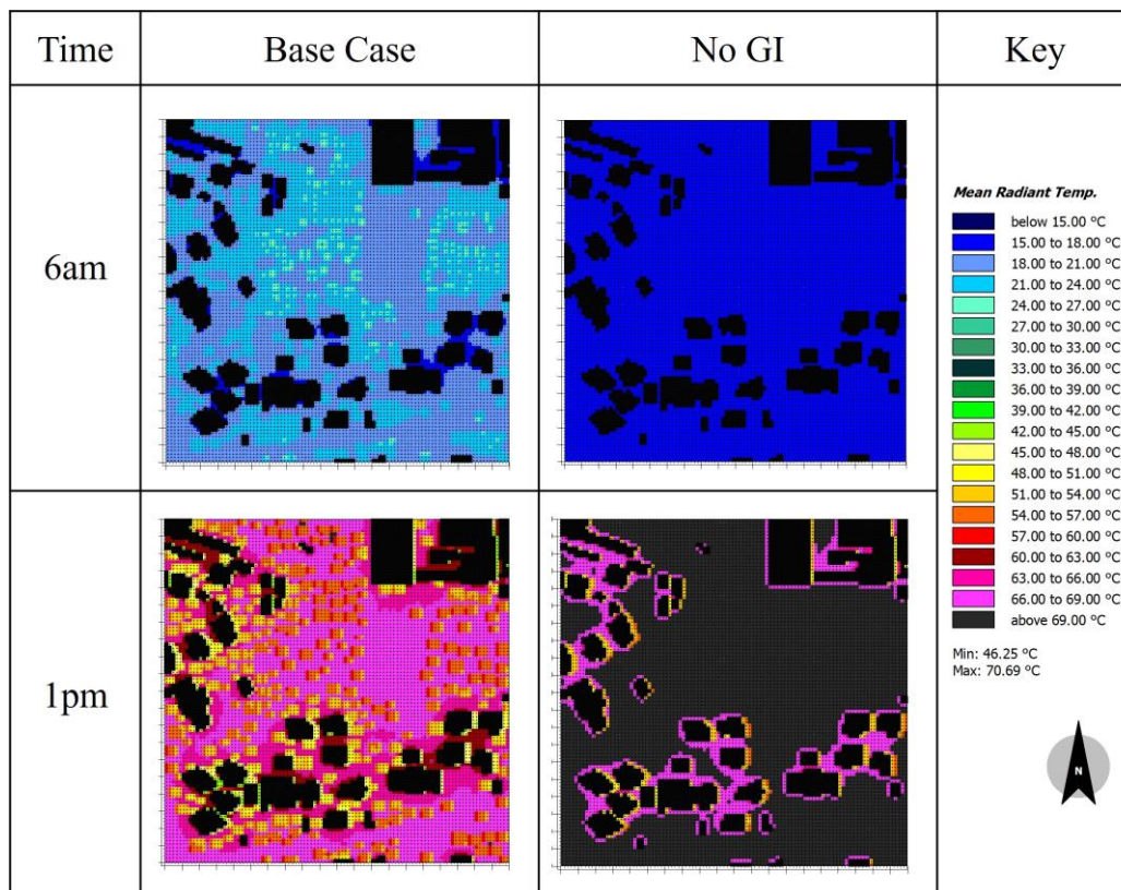
Figure 13. Spatial MRT variations at location 4 for 6 a.m. and 1 p.m.
