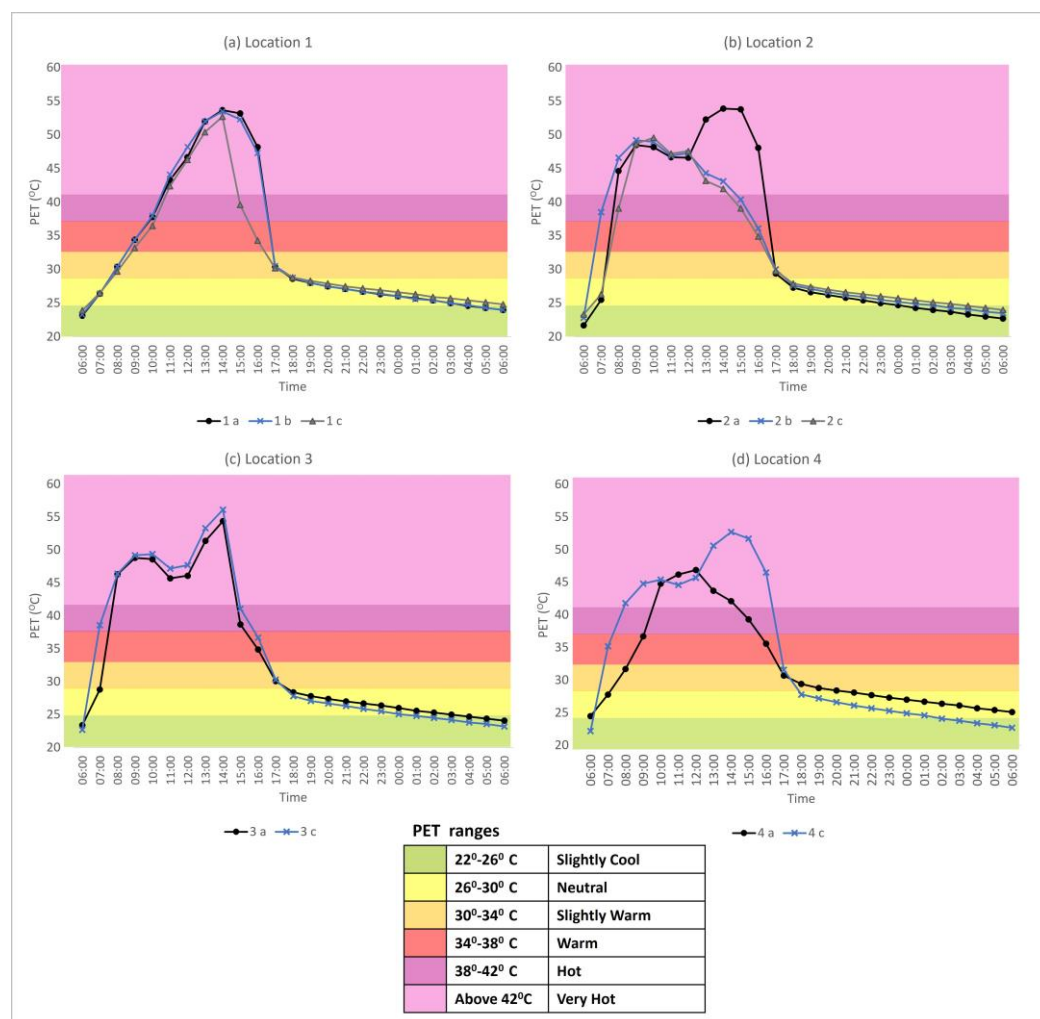
Figure 9. PET variation for the different scenarios on the simulated day.
