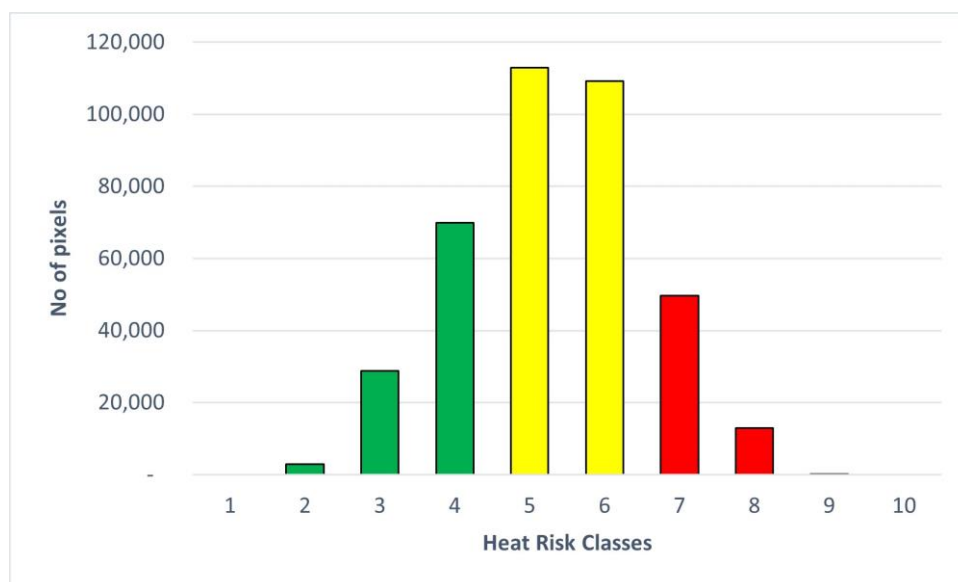
Figure 3. Distribution of heat risk classes.
