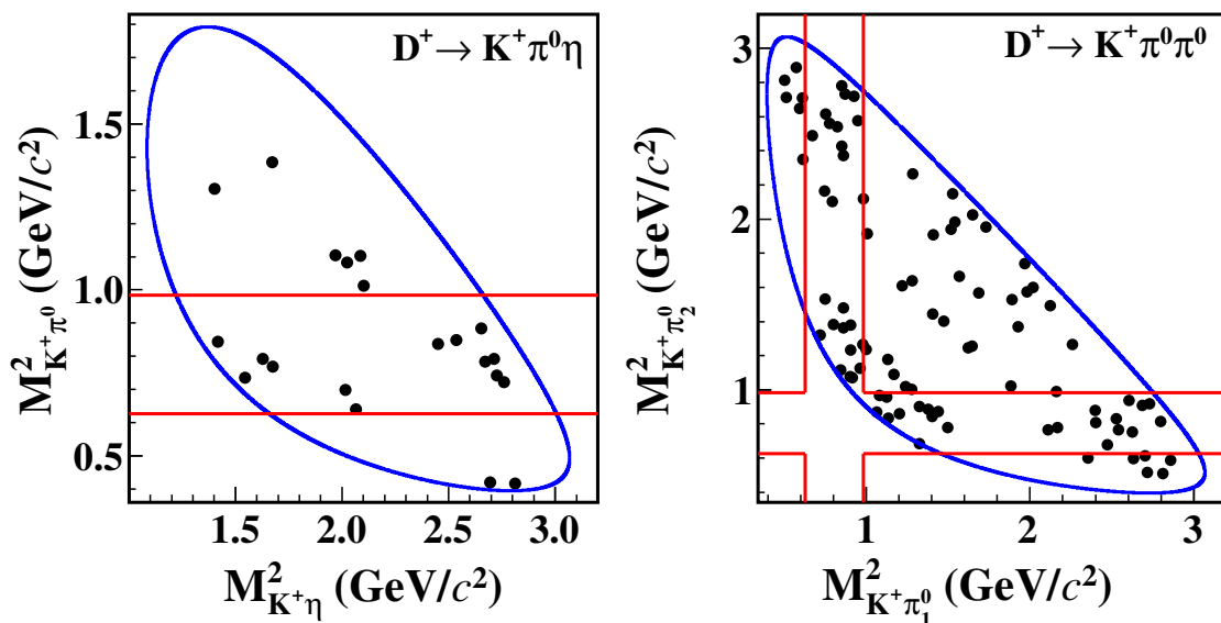
Figure 2. Distributions of (left) M_{K^+\pi^0}^2 versus M_{K^+\eta}^2 for D^+ \rightarrow K^+\pi^0\eta candidates and (right) M_{K^+\pi^0}^2 versus M_{K^+\pi_1^0}^2 for D^+ \rightarrow K^+\pi^0\pi^0 candidates (two entries per event for symmetrization). In the kinematic region marked in blue, the regions inside and outside the red band are the K^{*+} signal and sideband regions, respectively. The requirement of |M_{\text{BC}}^{\text{tag}(\text{sig})} - M_{D^+}| < 0.005 \text{ GeV}/c^2 has been imposed.
