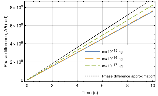
FIG. 4. Phase difference magnitude scaling with total runtime for m = 10^{-15} \text{ kg} , m = 10^{-16} \text{ kg} , and m = 10^{-17} \text{ kg} . This also shows the phase difference as predicted by Eq. (16).
