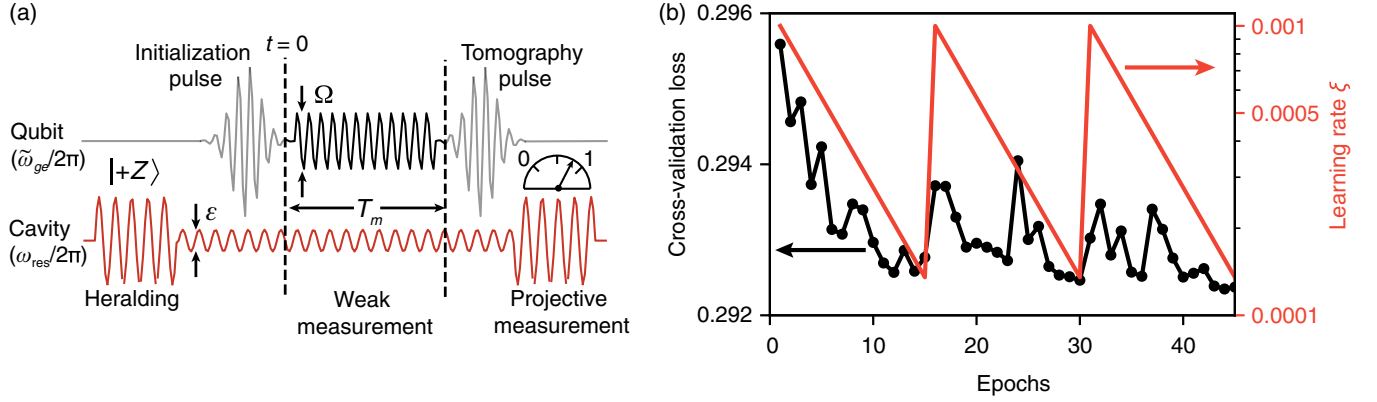
FIG. 7. (a) Experimental pulse sequence for training data acquisition. Time axis is not to scale. (b) Cost function (black, left-hand axis) computed on the cross-validation dataset during a typical training session. Temporary increases in the cost function are expected as the learning rate (red, right-hand axis) increases periodically.
