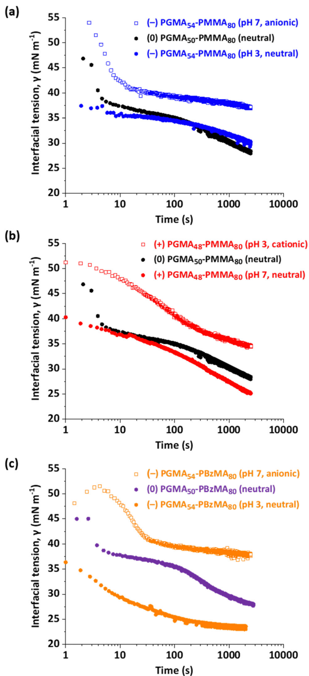
Fig. 4 Initial interfacial tension vs. time curves recorded for 20 \text{ nm}^3 droplets immersed in n -dodecane, where the droplet phase comprises the following 0.1% w/w aqueous copolymer dispersions. (a) (0) PGMA 50 -PMMA 80 nanoparticles prepared using the non-ionic PGMA 50 precursor and (–) PGMA 54 -PMMA 80 (pH 7, anionic) nanoparticles and (–) PGMA 54 -PMMA 80 (pH 3, neutral) nanoparticles prepared using the carboxylic acid-functionalized PGMA 54 precursor. (b) (0) PGMA 50 -PMMA 80 nanoparticles prepared using the non-ionic PGMA 50 precursor and (+) PGMA 48 -PMMA 80 (pH 3, cationic) nanoparticles and (+) PGMA 48 -PMMA 80 (pH 7, neutral) nanoparticles prepared using the morpholine-functionalized PGMA 48 precursor. (c) (0) PGMA 50 -PBzMA 80 nanoparticles prepared using the non-ionic PGMA 50 precursor, (–) PGMA 54 -PBzMA 80 (pH 7, anionic) nanoparticles and (–) PGMA 54 -PBzMA 80 (pH 3, neutral) nanoparticles prepared using the carboxylic acid-functionalized PGMA 54 precursor.
