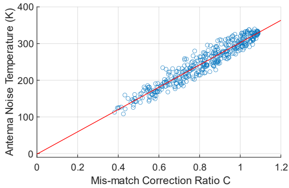
Fig. 1. Measured apparent antenna noise temperature against mis-match correction ratio C for an ambient temperature of 301 K.
