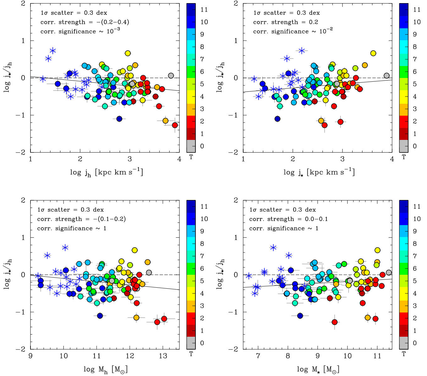
Figure A3. Same as Fig. A2, but for the fraction of specific angular momentum retained by the stellar component ( i_*/j_h ).
