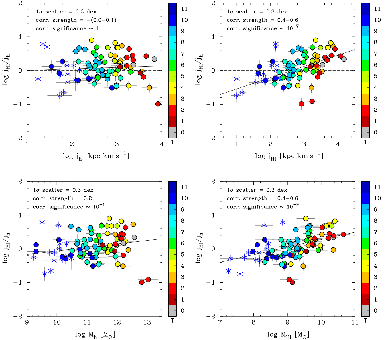
Figure A4. Same as Fig. A2, but for the fraction of specific angular momentum retained by the atomic gas component ( j_{\text{HI}}/j_{\text{h}} ).
