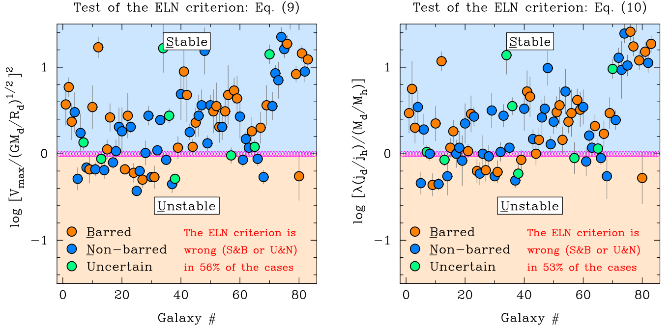
Figure B2. Additional test of the ELN criterion: the original criterion (Efstathiou et al. 1982 [equation (9)] versus the reformulation made by Mo et al. (1998) [equation (10)]. See Appendix B for more information.
