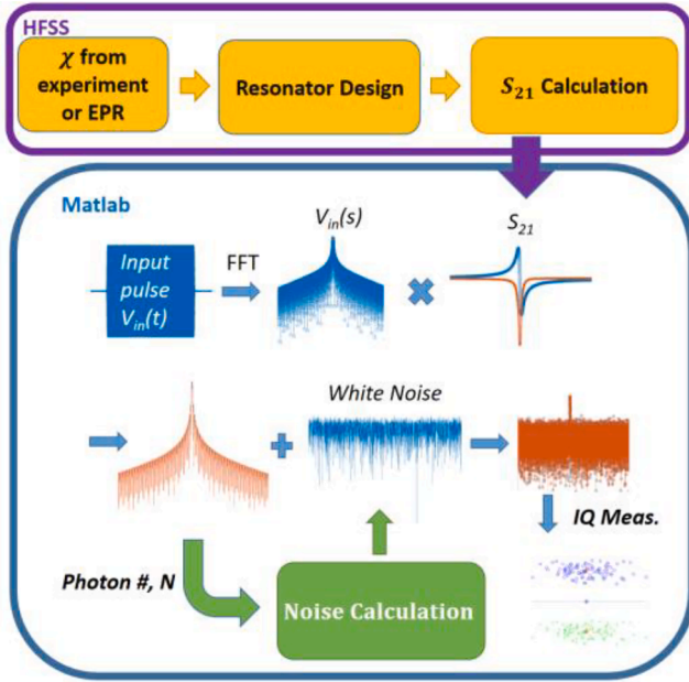
Fig. 2. Illustration of the simulation flow.
