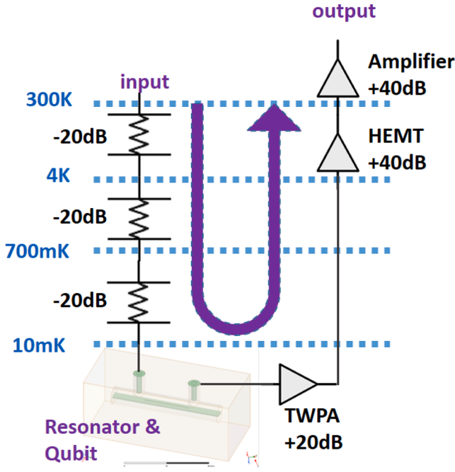
Fig. 1. The qubit system used. The readout path is highlighted.
