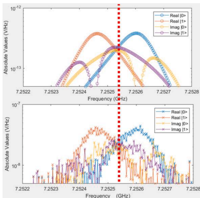
Fig. 4. The real and imaginary components of the signal after the resonator before adding the quantum noise (Top) and after the amplification chain in Fig. 1 (Bottom). The red dotted line indicates the reading pulse frequency. (For interpretation of the references to colour in this figure legend, the reader is referred to the web version of this article.)
