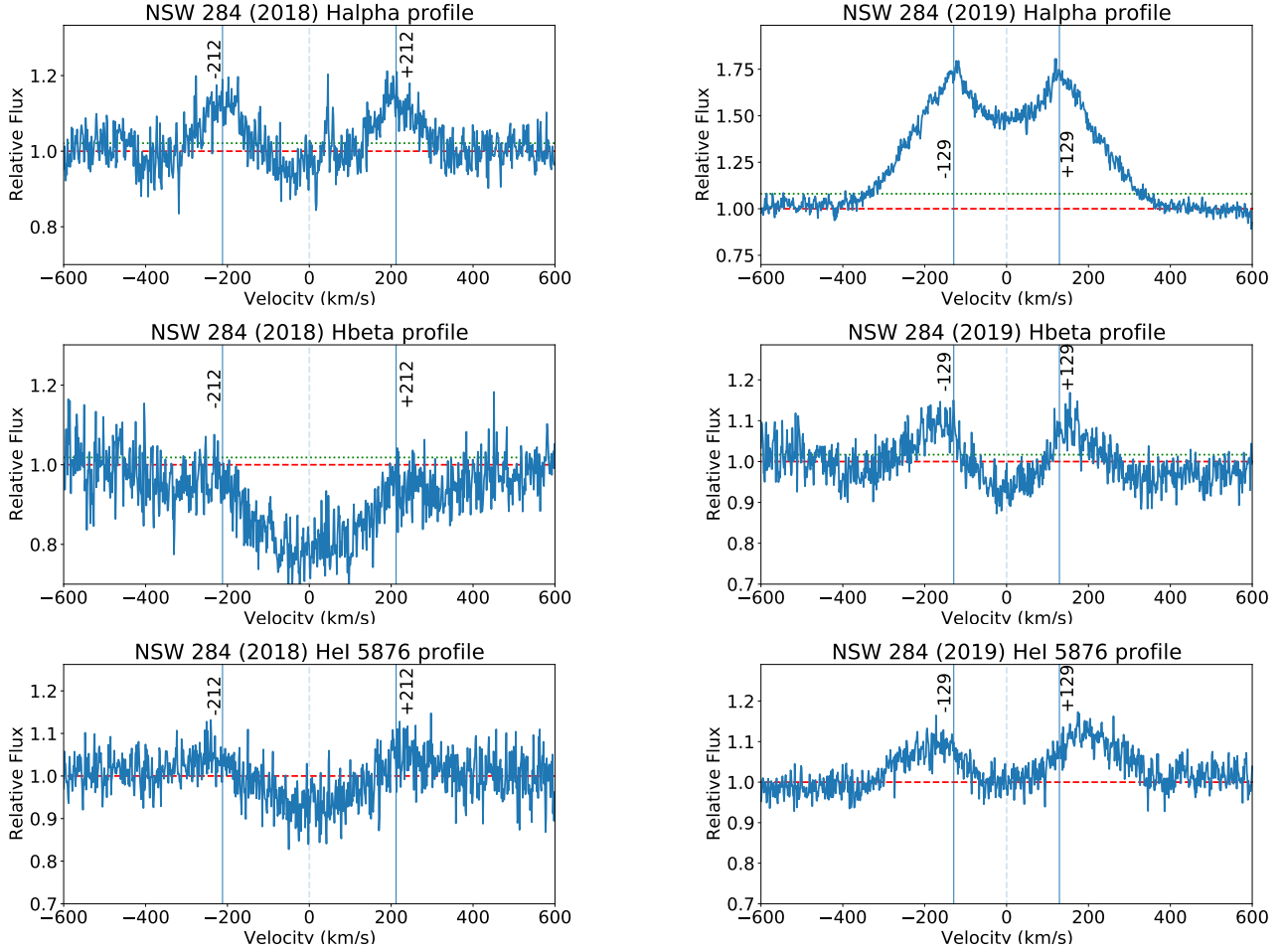
Figure 3. H\alpha , H\beta , and He I 5876 Å profiles for NSW 284 from 2018 (left, quiescence just after weak burst B4) and 2019 (right, during brightness decline of strong burst B5). The red dashed line shows the profile normalization level while the green dotted line indicates the 10% intensity. The vertical dashed line indicates zero stellocentric velocity, adopting a heliocentric radial velocity of -57.8 \text{ km s}^{-1} . Vertical lines at \pm 212 \text{ km s}^{-1} in 2018 and \pm 129 \text{ km s}^{-1} in 2019 correspond to the peaks of the double-horned profile in H\alpha . Note that the brighter photometric state corresponds to stronger lines but lower velocities. Note also that the peaks in H\beta seem to be at larger velocities than the peaks in H\alpha , and those in He I 5876 Å larger still.
