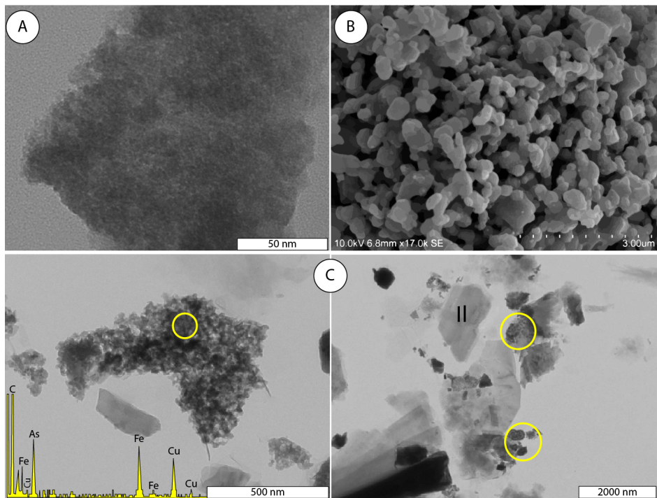
Figure 4 Images of ochre precipitates A, B – TEM and SEM micrographs of a 2-line ferrihydrite; C – TEM micrographs and EDS spectrum of iron and arsenic-rich nanoprecipitates, showing globular and spherical morphology (marked in yellow) associated with clay minerals; II - Illite.
