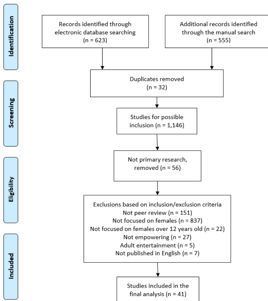
Figure 1. PRISMA Diagram
