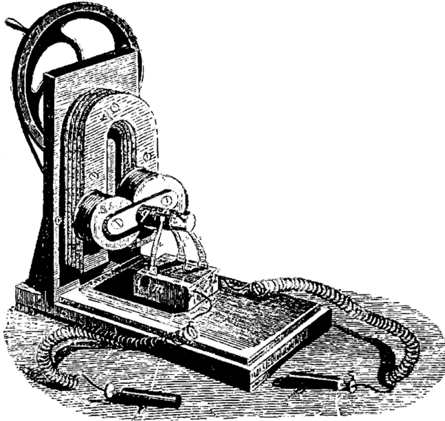
Figure 8. Clarke's magneto-electric apparatus (from Schivaldi P. (1868), p. 129).
