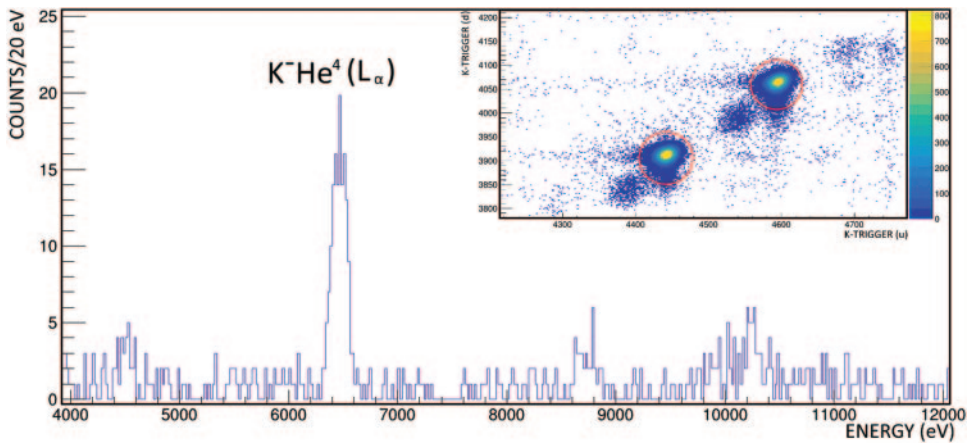
Fig. 2. – Preliminary calibrated spectrum of the first \text{K}^- \text{He}^4 \text{L}_\alpha transition measurement performed with the SIDDHARTA-2 experimental apparatus at the DAΦNE collider. On the top right inset, the kaon trigger 2D plot given by the coincidence signals detected by the scintillators allows the kaon selection (red circles).
