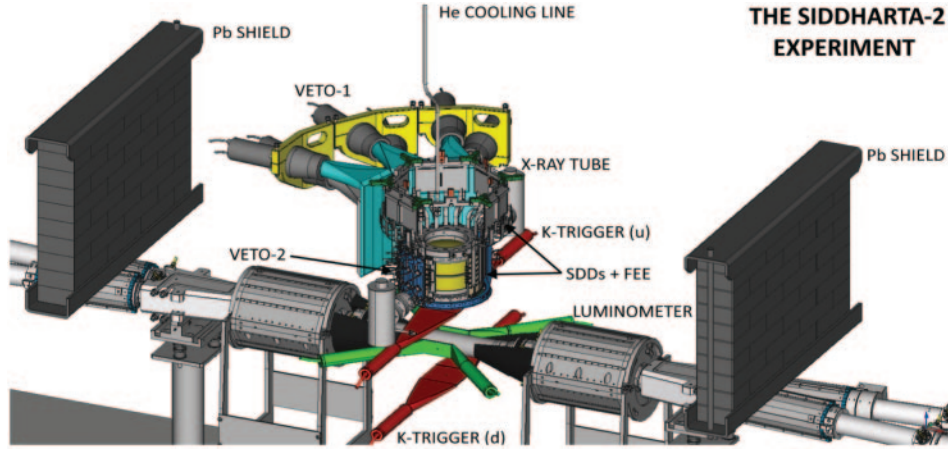
Fig. 1. – Layout of the SIDDHARTA-2 setup installed at the Interaction Region of the DAΦNE collider.
