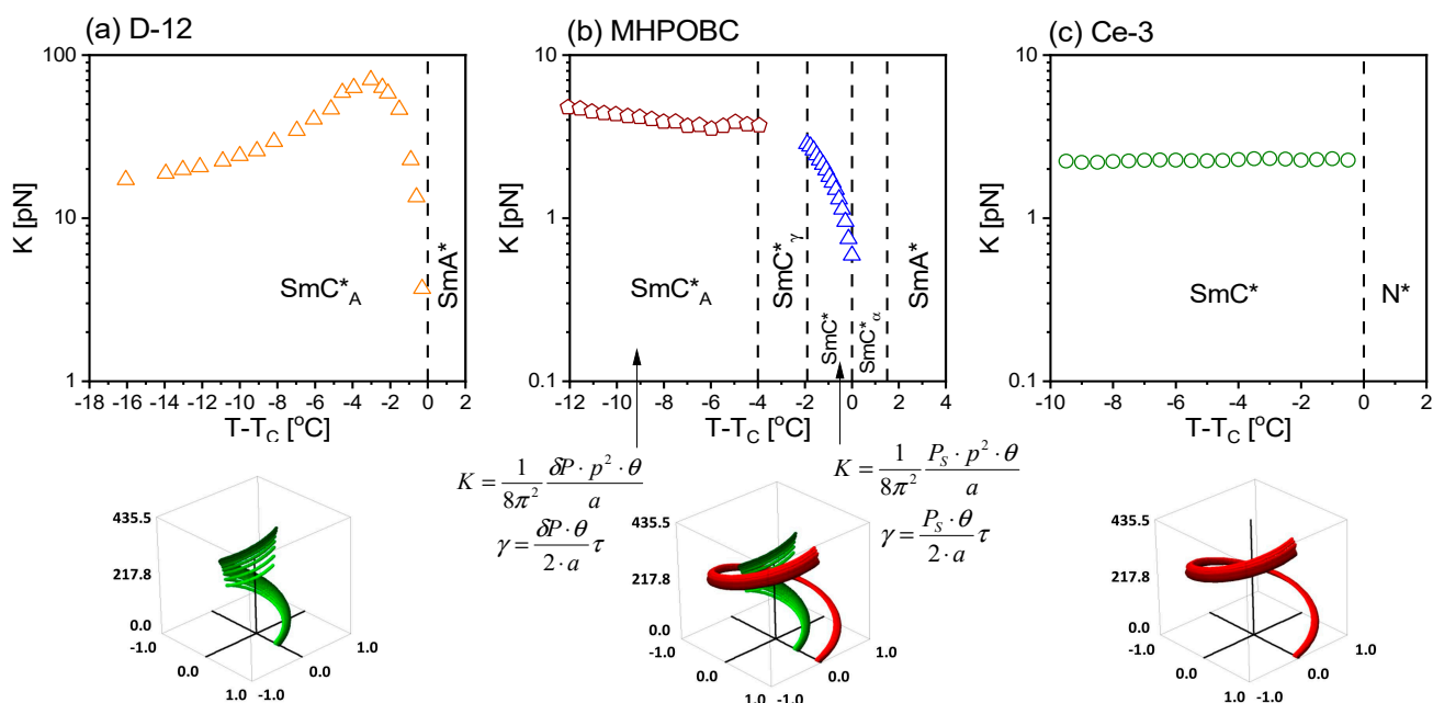
Figure 2. The elastic constant K versus temperature for three different materials in the low electric field range: (a) D-12, (b) MHPOBC and (c) Ce-3 showing different dependencies of the elastic constant depending on the type of adjacent phases. To illustrate the difference of the pitch behavior, schematic cartoons for one period of pitch for compounds are shown.
