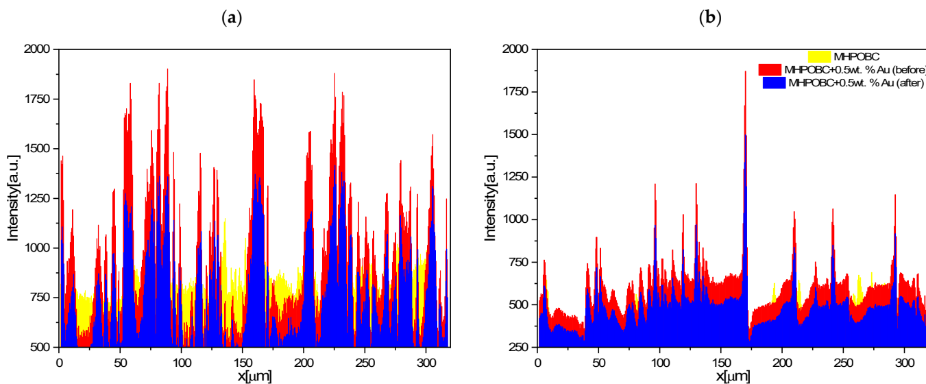
Figure 7. Fluorescence intensity versus horizontal dimension of pristine MHPOBC and MHPOBC doping with 0.5 wt.% Au NPs before and after photobleaching procedure, for detection in the blue (a) and green (b) light wavelength.
