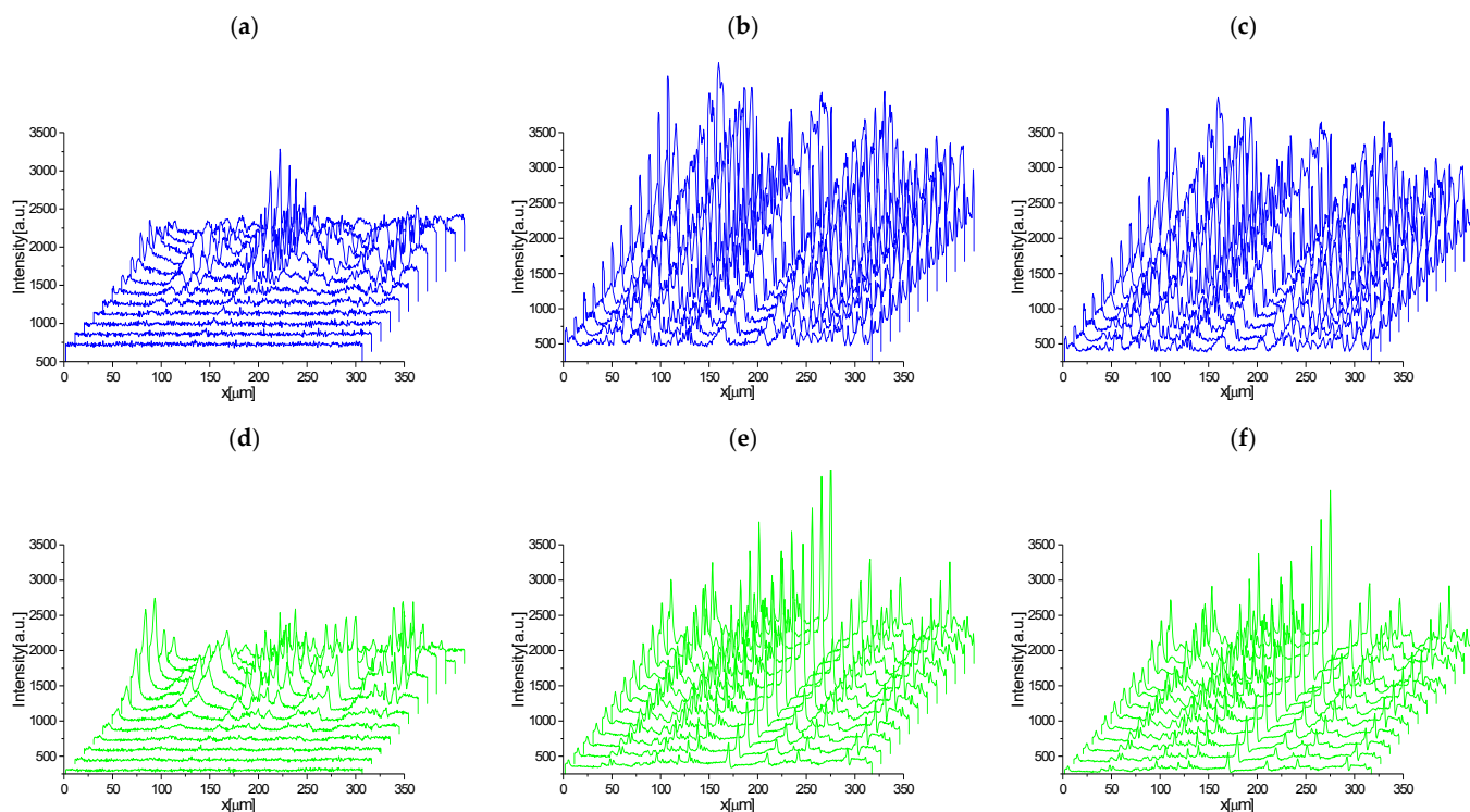
Figure 6. Fluorescence intensity versus horizontal dimension of the samples: pure MHPOBC liquid crystal (a,d), MHPOBC doping with 0.5 wt.% Au NPs before (b,e) and after (c,f) photobleaching procedure for detection in the blue and green light wavelength ranges, respectively. The third dimension represents successive scans taken as a function of cell thickness.
