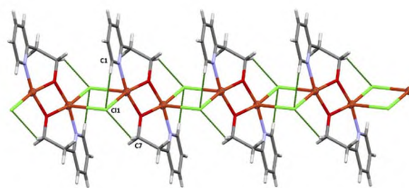
Fig. 6 Crystal packing diagram of 3 . The crystal packing analysis 24 revealed that the chains are stabilized by weak C–H...Cl interactions (see Table 5, figure).
