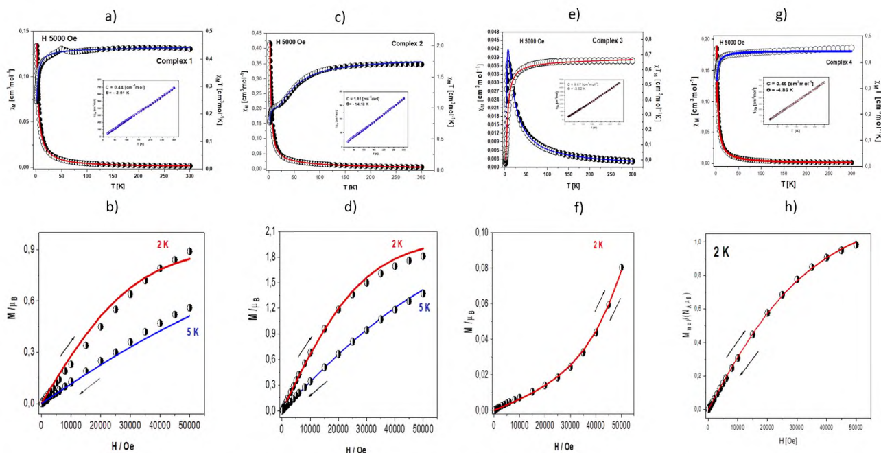
Fig. 10 Thermal dependencies of \chi_M T (open circles) and \chi_M (half-open circles) for (a) 1 , (c) 2 , (e) 3 and (g) 4 . The insets show thermal dependencies of inverse magnetic susceptibility. Magnetization as a function of the magnetic field for (b) 1 , (d) 2 , (f) 3 and (h) 4 . The solid lines (on all graphs) are calculated.
