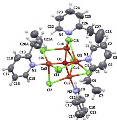
Fig. 3 Molecular structure of [\text{Cu}_4\text{OCl}_6(\text{ety})_4] together with the atom numbering. Displacement ellipsoids are drawn at 50% probability level.
