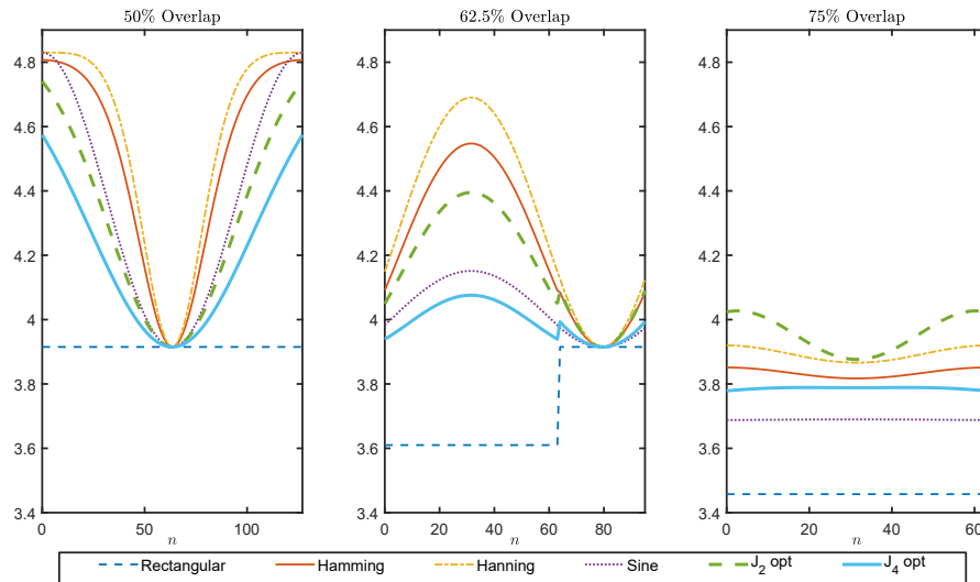
Figure 9: Time variations of the kurtosis for \beta_x = 4.83 and N = 256 . Left: 50% overlap; middle: 62.5% overlap; right: 75% overlap.
