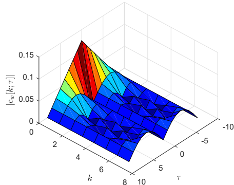
Figure 1: Magnitude of the Fourier coefficients c_w[k; \tau] for a rectangular window of length N = 8 and no overlap ( D = N ), indicating significant non-stationarity.
