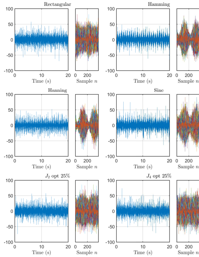
Figure 7: Time realization (left) and overlay of blocks of 256 samples length (right) of a white random process with kurtosis \bar{\beta}_z = 4.83 and N = 256 , using different synthesis windows and 25% overlap.
