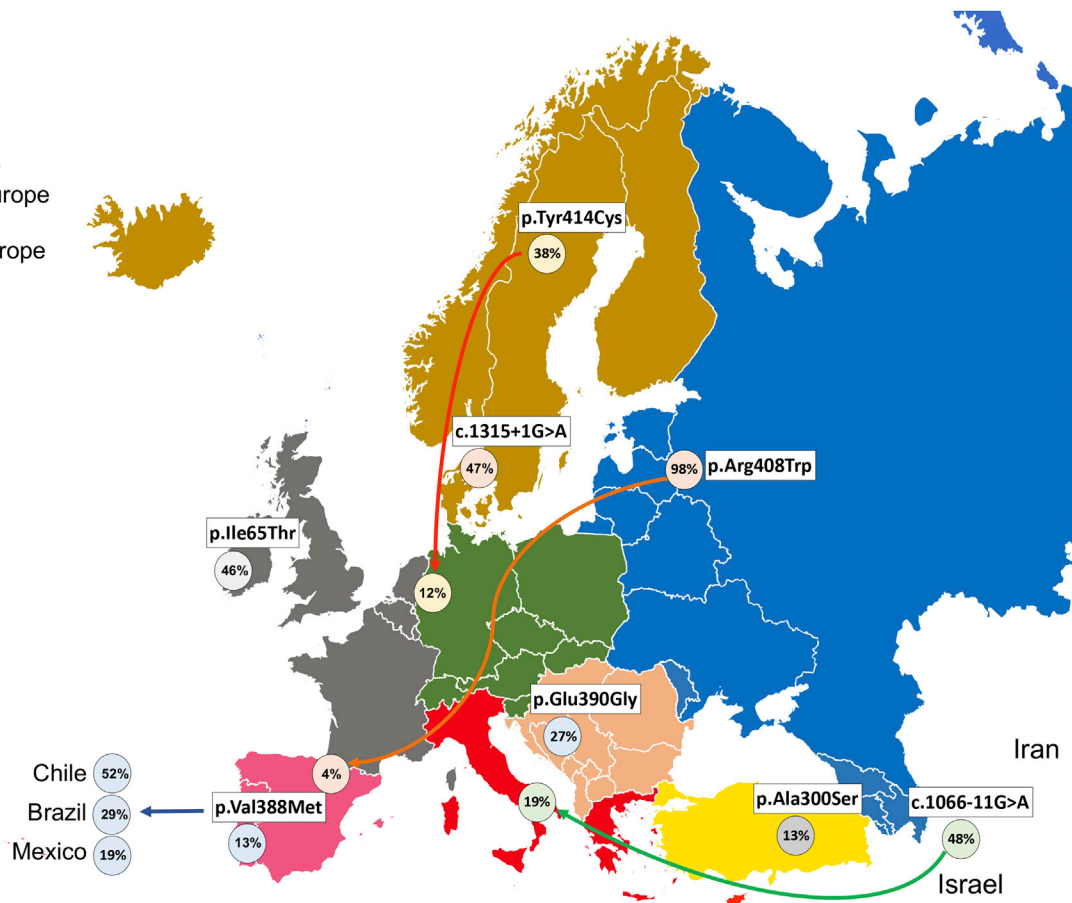
Figure 5. Patterns of Common PAH Variants Possibly Associated with Migration in Europe
