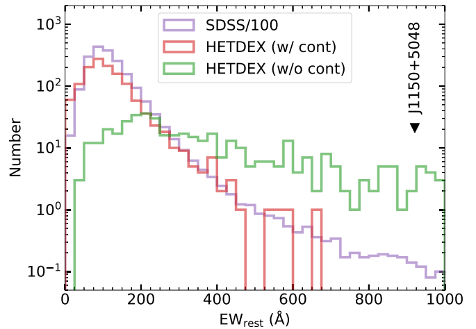
Figure 1. Distributions of the rest-frame EW of the Ly\alpha + N\ V\ \lambda 1241 emission. HETDEX AGNs with continuum detection ( >1\sigma ) are shown in the red histogram. HETDEX AGNs without continuum detection ( <1\sigma ) are shown in the green histogram. SDSS quasars are indicated by purple histogram. The number of SDSS quasars in each bin is divided by 100 for presentation purposes. EW_{(Ly\alpha+N\ V),rest} of J1150+5048 is marked by the downward triangle.
