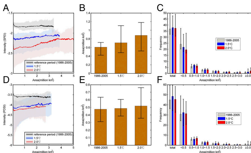
Fig. 2. Averaged drought intensity at different contiguous drought areas ( A and D ), averaged coverage of drought events ( B and E ), and annual frequency of drought events with different coverage ( C and F ) in China for the 1.5 °C and 2.0 °C global warming period and the reference period (1986–2005). Drought characteristics in A – C and D – F are deduced by the SPEI and PDSI, respectively. Shadows and lines in A and D are the bands and median, respectively, for 22 GCM runs. Histograms and black vertical lines in B and C and E and F denote the median and range of multimodel projections, respectively.
