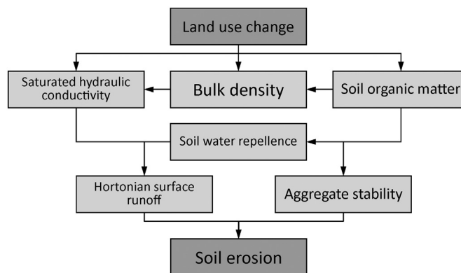
Fig. 6. Specific interdependencies between land use changes, soil properties and soil erosion in the Onsernone valley. Arrows indicate the direction of influence.
