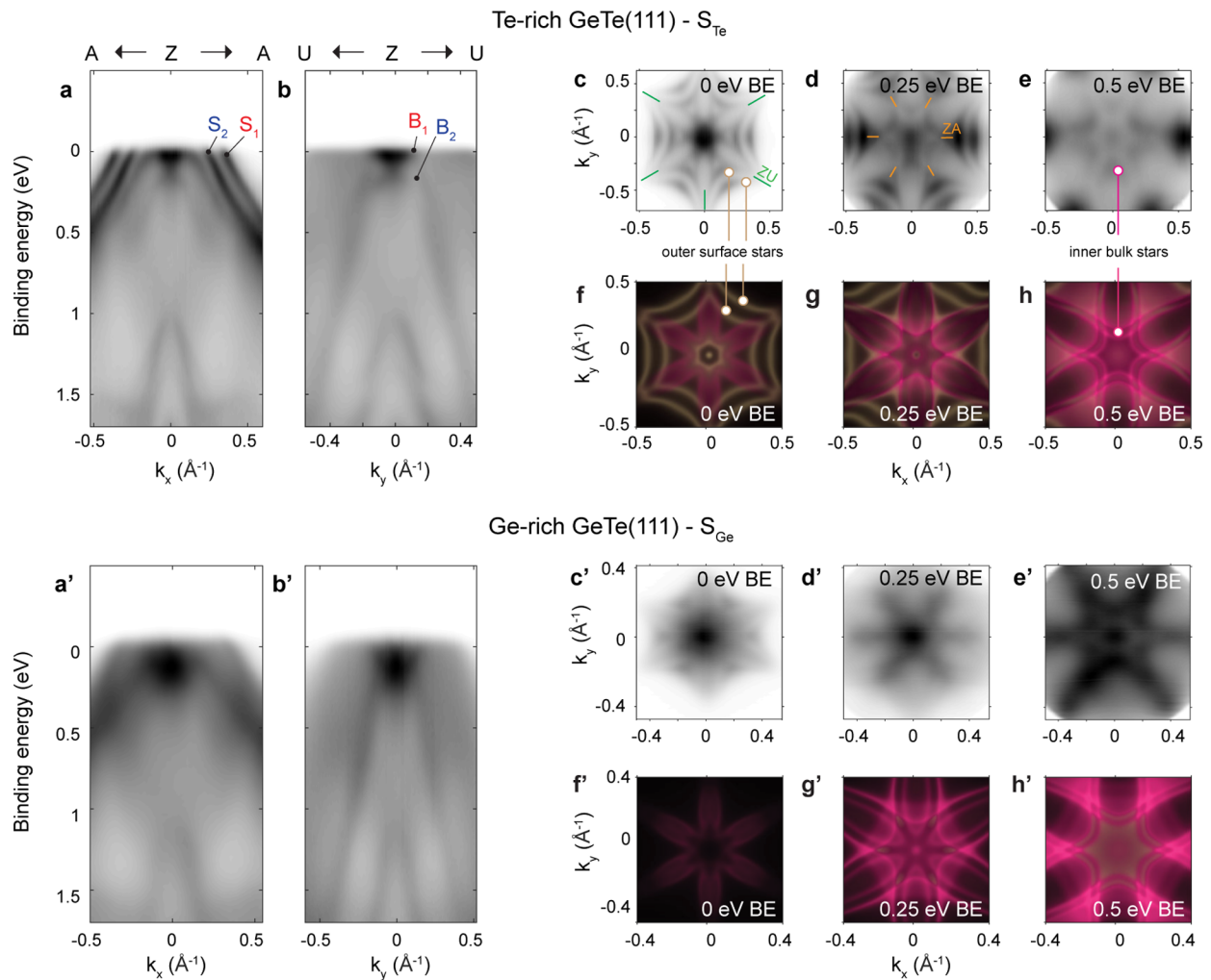
Figure 3. ARPES from Te-rich and Ge-rich samples. Panels a–h refer to the Te-rich sample S_{\text{Te}} with outward polarization. (a, b) Experimental bands dispersion collected along the principal directions ZA ( k_x ) and ZU ( k_y ) in the Brillouin zone. (c–e) Constant energy maps at 0, 0.25, and 0.5 eV below the Fermi energy. (f–h) Corresponding calculated constant energy maps with yellow and pink indicating the surface and bulk character of states, respectively. Panels labeled by the apex (panels a'–h') are the same as above but for the Ge-rich sample S_{\text{Ge}} with inward polarization. The Fermi level in panels f'–h' is chosen to be consistent with Figure 2.
