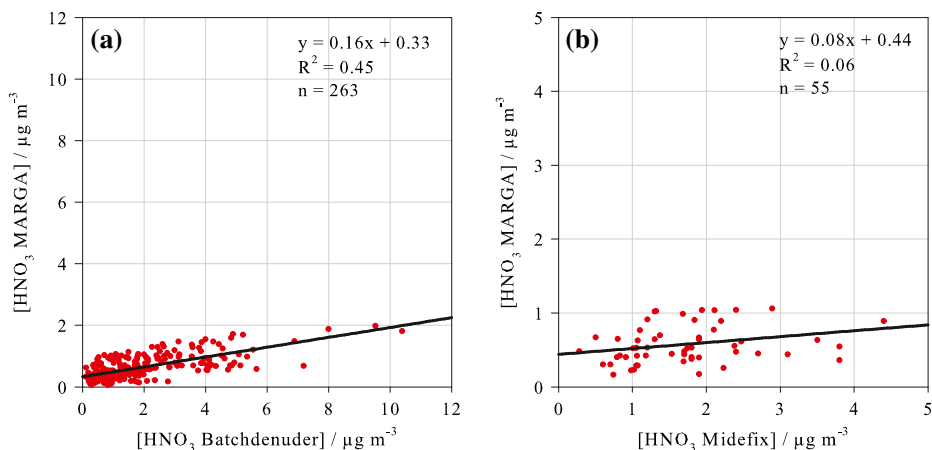
Fig. 4 Comparison of \text{HNO}_3 measurements with the MARGA ( y -axis) and (a) the rotating annular batch denuder and (b) Midefix, orthogonal regression ( black line )
