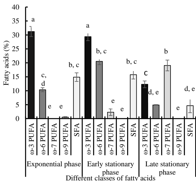
Figure 6. Major fatty acids in methanol extracts at various growth phases of microalgae; omega-3 and omega-6 as PUFAs, omega-7 and omega-9 as MUFAs and all of the saturated fatty acids (SFA) as one group. Proportional distribution of individual fatty acids is associated to the total content. a-e Mean values with similar letters are statistically similar, while mean values with different letters are significantly different using Tukey test ( p \leq 0.05 )
