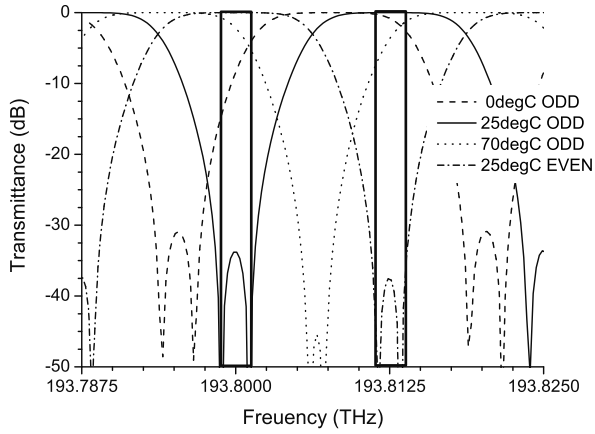
Fig. 4: Calculated characteristics of temperature changing of the interlever at 25°C and 1013 hPa.
