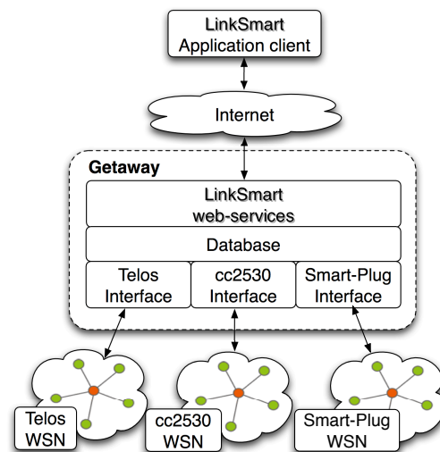
Fig. 1. Software infrastructure scheme to handle heterogeneous wireless sensor networks.
