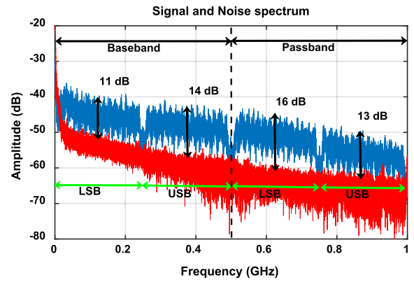
Fig. 10. Signal spectrum at the ADC input when both SWs are active.
