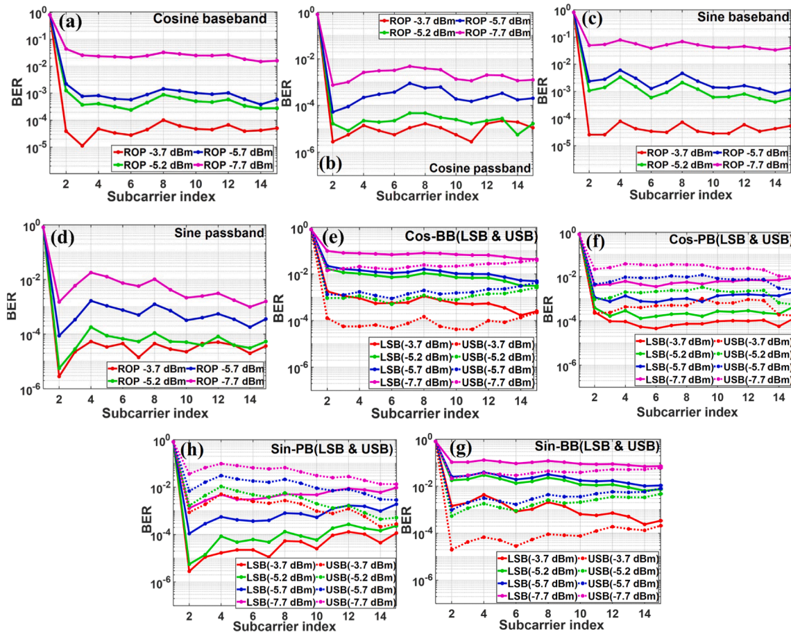
Fig. 12. BER vs subcarrier index for (a) cosine baseband (JSP) (b) cosine passband (JSP) (c) sine baseband (JSP) (d) sine passband (JSP) (e) Cos-BB (LSB & USB) (f) Cos-PB (LSB & USB) (g) Sin-BB (LSB & USB) and (h) Sin-PB (LSB & USB).
