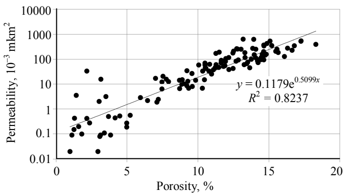
Fig. 2. Dependence K_{pr} = f(K_p) for deposits of the Middle Devonian Afoninsky horizon
