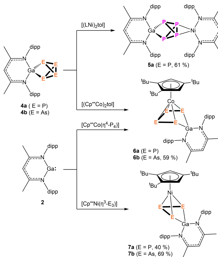
Scheme 3. Reaction of 4 with unsaturated transition metal complexes and reaction of 2 with E_n ligand complexes (dipp = 2,6-diisopropylphenyl, Cp''' = C_5H_2tBu_3 ).
