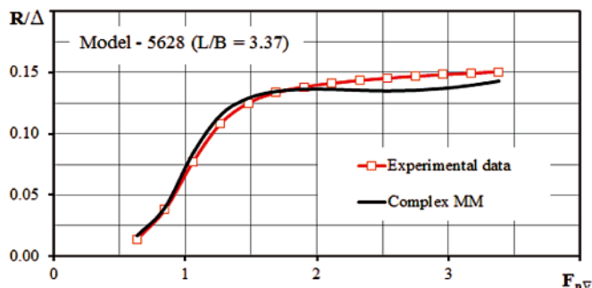
Fig. 36. Discrepancies between evaluated and tested R/\Delta data of USC models 5630, 5629 and 5628
