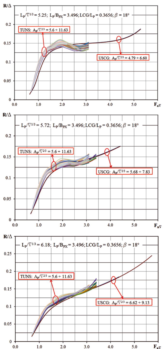
Fig. 5. Typical R/\Delta values in the overlapping zone
