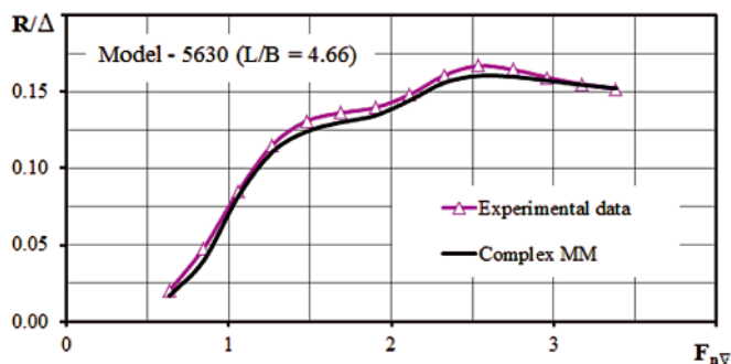
Fig. 34. The influence of L/B on R/\Delta
