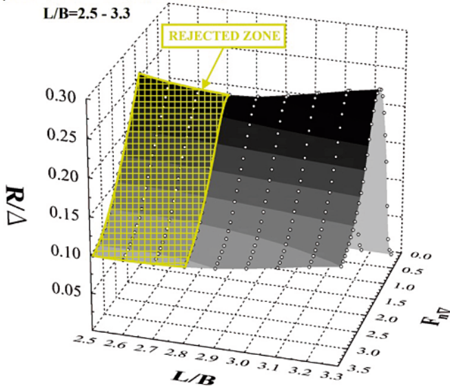
Fig. 24. Reduction of the applicability zone due to saddle
