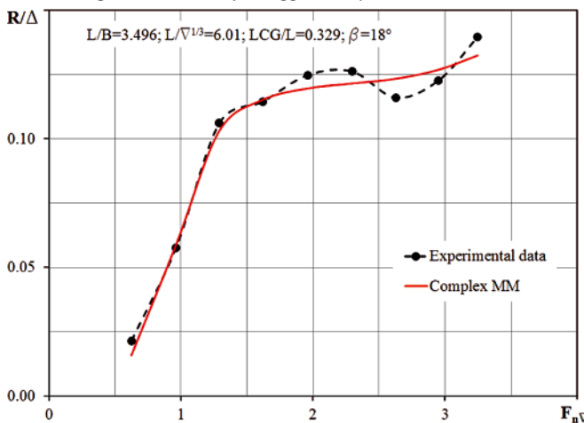
Fig. 25. R/\Delta tested and evaluated in the middle of applicability zone
