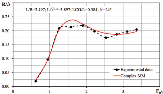
Fig. 19. R/\Delta tested and evaluated on applicability boundaries
