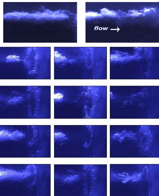
Figure 13. Images of the 2 nd and 3 rd part of cavitating jet obtained using NAVITAR magnifier lenses (first two images are for the 2 nd part) (NAVITAR 2x adapter (1-6010)(1-6030) (1-60135)). (Gain = 600 V, shutter time = 1 \mu s, Conditions: p_1=164 bar, p_2=3.04 bar, v_j=156 m/s, \sigma = 0.025 , T=18^\circ\text{C} ).
