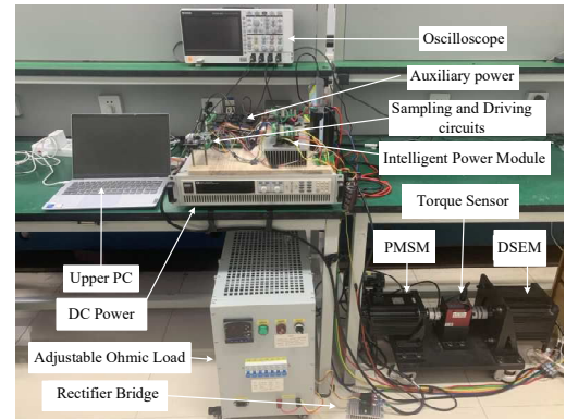
Fig. 11. Experimental prototype
