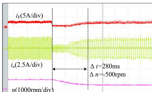
T/(100ms/div) (b) Decelerate
