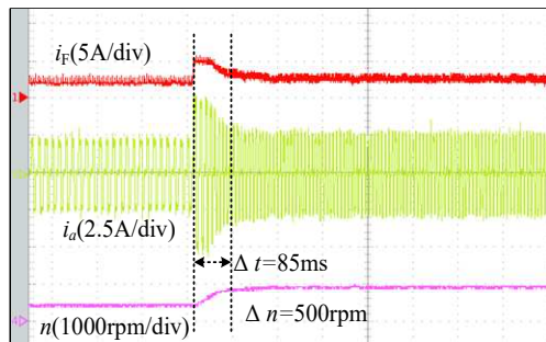
T/(100ms/div) (a) Accelerate
