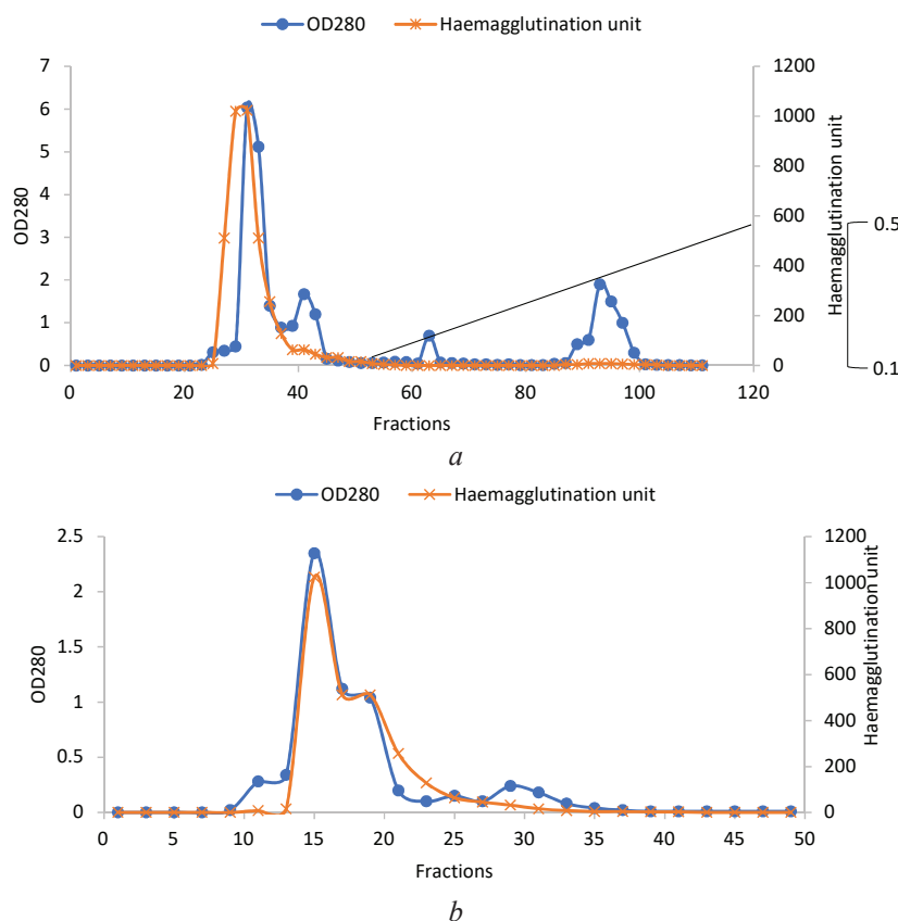
Fig. 2. Column chromatography profile of Treculia africana seed lectin: a – Ion-exchange chromatography of T. africana seed crude extract on DEAE-cellulose column (elution buffer: 0.025 PBS, pH 7.2. Adsorbed protein was eluted with a linear gradient of 0.1 – 0.5 M NaCl in phosphate-buffered saline; column size: 1.6 \times 40 cm; flow rate: 24 ml/h; fraction volume: 2 ml); b – Gel filtration of pooled fractions from ion-exchange on Sephadex G-100 (elution buffer: 0.025 PBS; column size: 1.5 \times 63 cm; flow rate: 20 ml/h; fraction volume: 4 ml)
