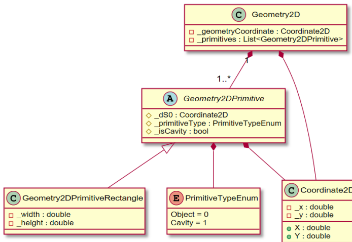
Fig. 1. Class diagram for describing the geometry of the object under study.
