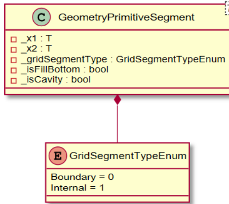
Fig. 2. Geometry segment class diagram.
