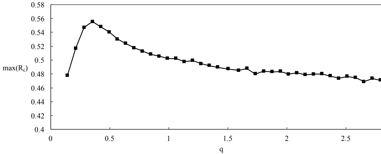
FIGURE 9. Maximum of the average order parameter in the locally locked state \max(R_C) depending on q fixing L = 1, \Delta x = 0.05, N = 400 , applying first order kernel-function. For the simplicity, the diagram was computed assuming IC 1.
