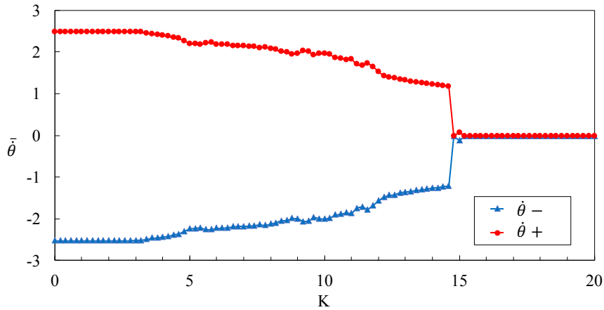
FIGURE 6. Average frequency in the function of the coupling strength for the sub-populations corresponding to \Omega_i < 0 ( \bar{\theta}_i^- ) and \Omega_i \geq 0 ( \bar{\theta}_i^+ ) for IC 1 taking the same parameters as in Fig. 2c.
