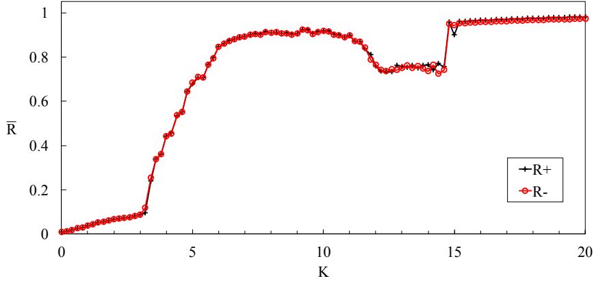
FIGURE 5. Average order parameter in the function of the coupling strength for the sub-populations corresponding to \Omega_i < 0 (R-) and \Omega_i \geq 0 (R+) for IC 1 taking the same parameters as in Fig. 2c.
