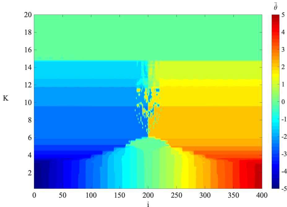
FIGURE 3. Average frequency \bar{\theta} in the function of the oscillator index i and the coupling strength K .
