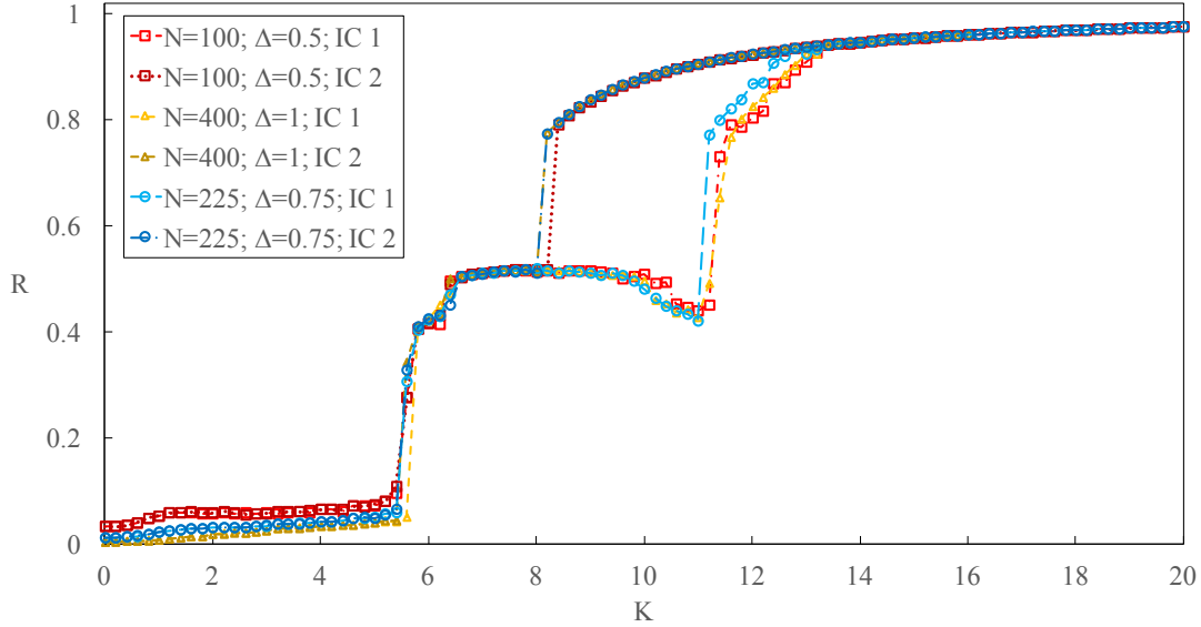
FIGURE 8. Average order parameter \bar{R} versus the coupling parameter K calculated for IC 1 and IC 2, fixing q \approx 0.7 , and changing both the kernel radius and the domain size: \Delta_1 = L_1 = 0.5, \Delta_2 = L_2 = 0.75, \Delta_3 = L_3 = 1 , applying the first order kernel W_{ij}^1 .
