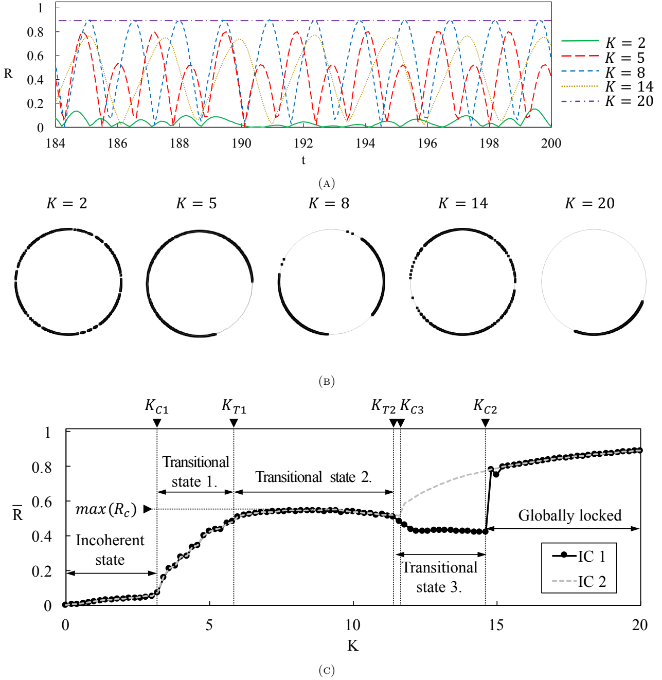
FIGURE 2. States of a system of spatially coupled oscillators depending on the coupling parameter K . The relative kernel radius is q \approx 0.46 , taking \Delta = 0.6 and \Delta x = 0.05 , N = 400 applying first order kernel-function. a) Time series of the order parameter R for different values of K calculated for IC 1. For K_{C1} < K < K_{C2} , R has an oscillatory nature. b) Final phases of the oscillators in polar form at t = 500s illustrating the different states of the system calculated for IC 1. c) States of the system and the time average \bar{R} of the order parameter depending on the coupling parameter K .
