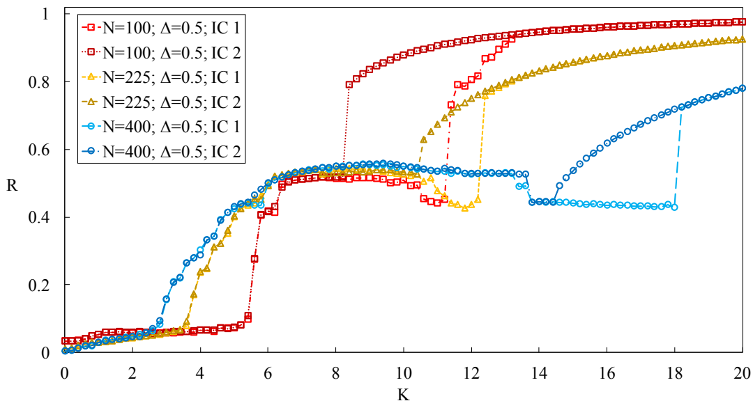
FIGURE 7. Average order parameter \bar{R} versus the coupling parameter K calculated for IC 1 and IC 2 fixing the kernel radius \Delta = 0.5 and varying the domain size L_1 = 0.5, L_2 = 0.75, L_3 = 1 ( q_1 \approx 0.7, q_2 \approx 0.47, q_3 \approx 0.35 ), applying the first order kernel W_{ij}^1 .
