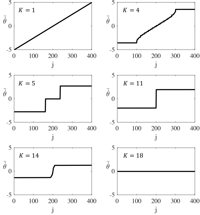
FIGURE 4. Average frequency \bar{\theta} of the oscillators for different K values, ordered for increasing frequency values. j is the oscillator index after reordering for each K values. For small K values, the system is in an unsynchronized state ( K = 1 ), then for increasing K locally locked clusters develop and merge ( K = 4 and K = 5 ) until there are only two separated clusters ( K = 11 ) which start to merge ( K = 14 ) and finally there is only one cluster ( K = 18 ).
