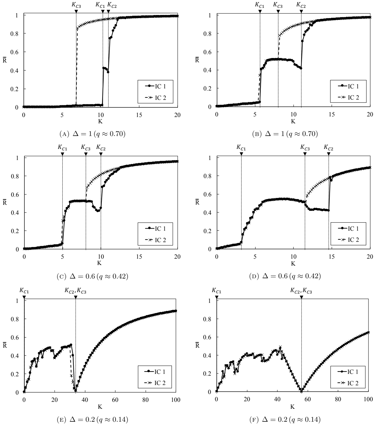
FIGURE 1. Comparison of the hysteric loops of synchronization in case of different kernel radii. Results with zeroth and first order kernel-functions are shown on the left and right, respectively.
